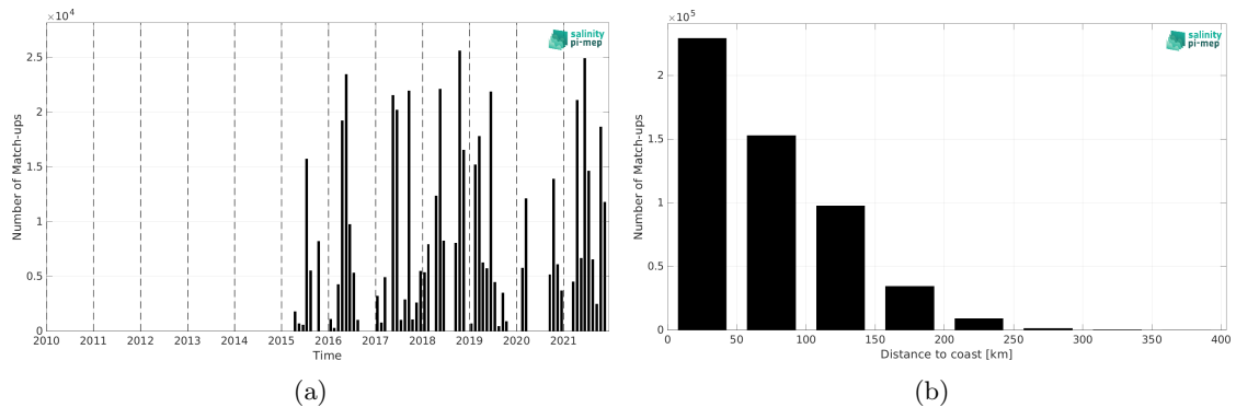
Figure 2: Number of match-ups between TSG (GOSUD-Research-vessel) and SMAP SSS L3 v6 - Monthly (RSS) SSS as a function of time (a) and as function of the distance to coast (b) over the Mediterranean Sea Pi-MEP region and for the full satellite product period.
