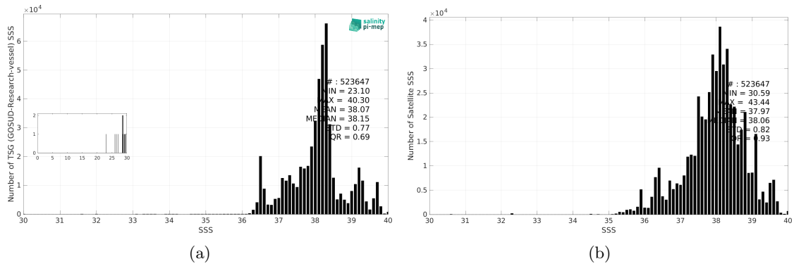
Figure 3: Histograms of SSS from TSG (GOSUD-Research-vessel) (a) and SMAP SSS L3 v6 - Monthly (RSS) (b) considering all match-up pairs per bins of 0.1 over the Mediterranean Sea Pi-MEP region and for the full satellite product period.
