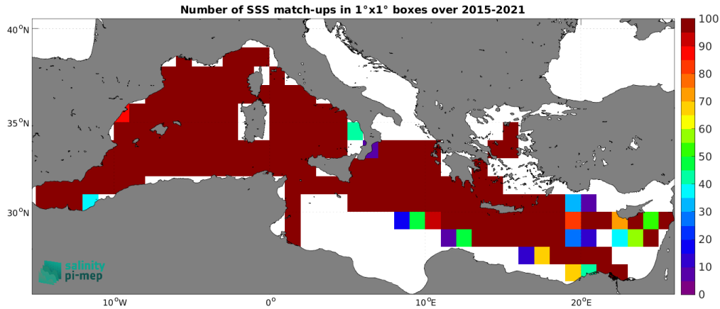
Figure 5: Number of SSS match-ups between TSG (GOSUD-Research-vessel) SSS and the SMAP SSS L3 v6 - Monthly (RSS) SSS product for the Mediterranean Sea Pi-MEP region over 1^\circ \times 1^\circ boxes and for the full satellite product period.
