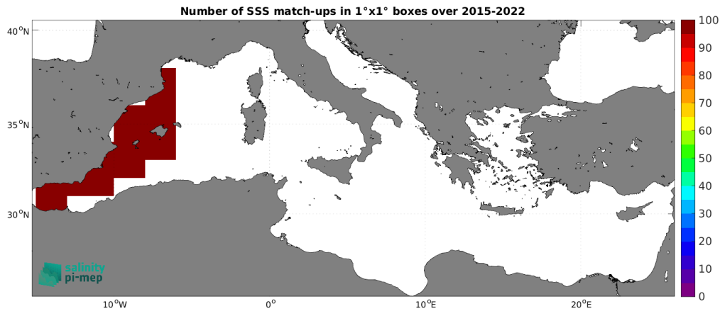
Figure 5: Number of SSS match-ups between TSG (CSIC-UTM) SSS and the SMAP SSS L3 v6 - Monthly (RSS) SSS product for the Mediterranean Sea Pi-MEP region over 1^\circ \times 1^\circ boxes and for the full satellite product period.
