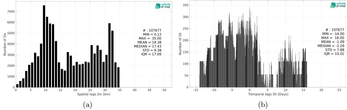
Figure 6: Histograms of the spatial (a) and temporal (b) lags between the location/time of the TSG (CSIC-UTM) measurement and the date of the corresponding SMAP SSS L3 v6 - Monthly (RSS) SSS pixel.
