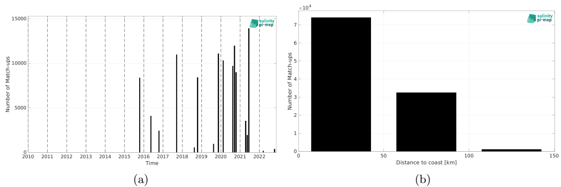
Figure 2: Number of match-ups between TSG (CSIC-UTM) and SMAP SSS L3 v6 - Monthly (RSS) SSS as a function of time (a) and as function of the distance to coast (b) over the Mediterranean Sea Pi-MEP region and for the full satellite product period.
