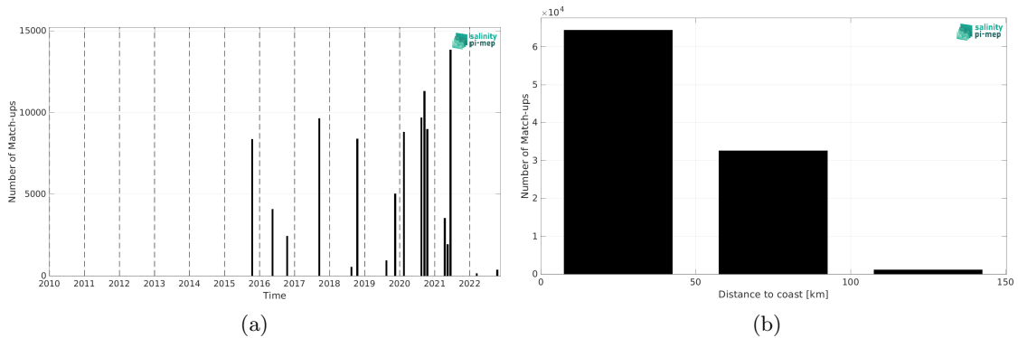
Figure 2: Number of match-ups between TSG (CSIC-UTM) and SMAP SSS L3 v5.3 - 8-Day running (RSS) SSS as a function of time (a) and as function of the distance to coast (b) over the Mediterranean Sea Pi-MEP region and for the full satellite product period.
