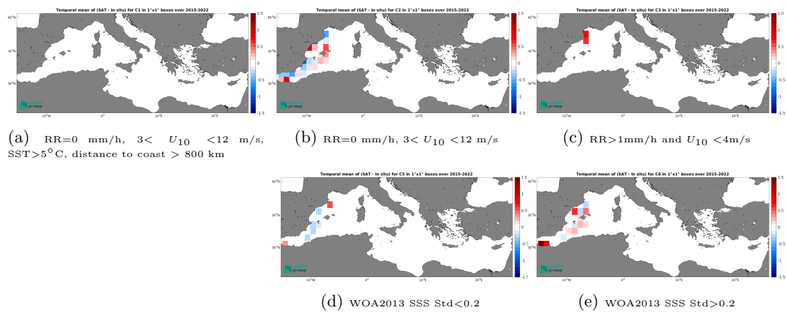
Figure 14: Temporal mean gridded over spatial boxes of size 1^\circ \times 1^\circ of \Delta\text{SSS} (SMAP SSS L3 v5.3 - 8-Day running (RSS) - TSG (CSIC-UTM)) for 5 different subdatasets corresponding to:RR=0 mm/h, 3 < U_{10} < 12 m/s, SST>5°C, distance to coast > 800 km (a), RR=0 mm/h, 3 < U_{10} < 12 m/s (b), RR>1mm/h and U_{10} < 4 m/s (c), WOA2013 SSS Std<0.2 (d), WOA2013 SSS Std>0.2 (e).
