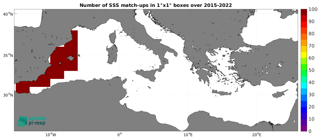
Figure 5: Number of SSS match-ups between TSG (CSIC-UTM) SSS and the SMAP SSS L3 v5.3 - 8-Day running (RSS) SSS product for the Mediterranean Sea Pi-MEP region over 1^\circ \times 1^\circ boxes and for the full satellite product period.
