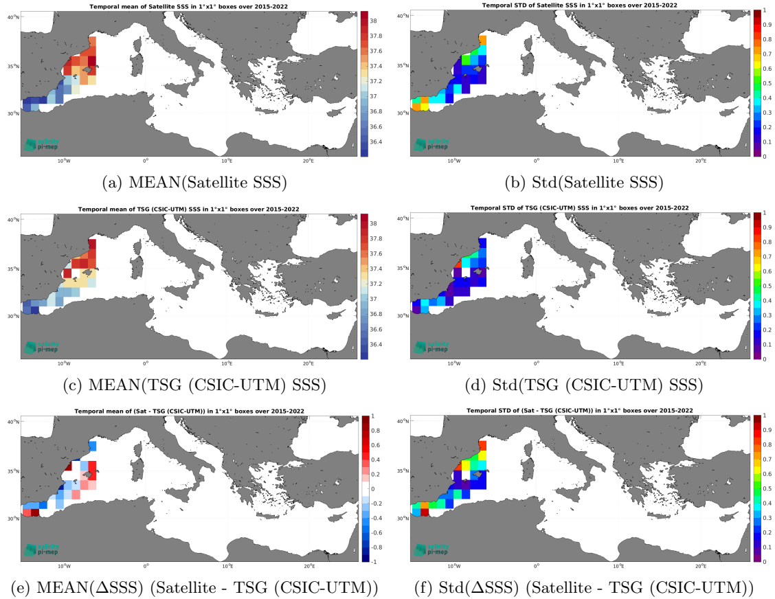
Figure 7: Temporal mean (left) and Std (right) of SSS from SMAP SSS L3 v5.3 - 8-Day running (RSS) (top), TSG (CSIC-UTM) (middle), and of \Delta\text{SSS} (Satellite - TSG (CSIC-UTM)). Only match-up pairs are used to generate these maps.
