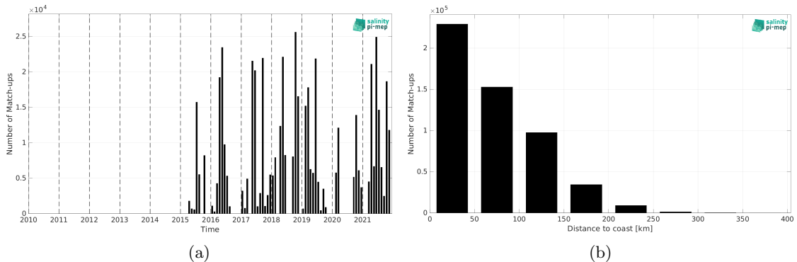
Figure 2: Number of match-ups between TSG (GOSUD-Research-vessel) and SMAP SSS L3 v5.3 - Monthly (RSS) SSS as a function of time (a) and as function of the distance to coast (b) over the Mediterranean Sea Pi-MEP region and for the full satellite product period.
