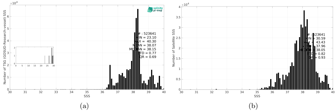
Figure 3: Histograms of SSS from TSG (GOSUD-Research-vessel) (a) and SMAP SSS L3 v5.3 - Monthly (RSS) (b) considering all match-up pairs per bins of 0.1 over the Mediterranean Sea Pi-MEP region and for the full satellite product period.
