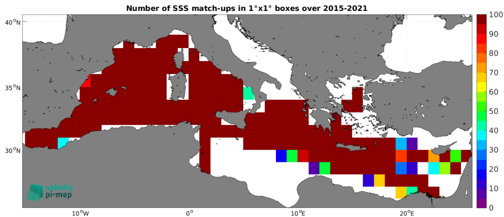
Figure 5: Number of SSS match-ups between TSG (GOSUD-Research-vessel) SSS and the SMAP SSS L3 v5.3 - Monthly (RSS) SSS product for the Mediterranean Sea Pi-MEP region over 1^\circ \times 1^\circ boxes and for the full satellite product period.
