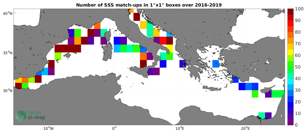
Figure 4: Number of SSS match-ups between TSG (GOSUD-Sailing-ship) SSS and the SMAP SSS L3 v5 - 8-Day running (RSS) SSS product for the Mediterranean Sea Pi-MEP region over 1^\circ \times 1^\circ boxes and for the full satellite product period.
