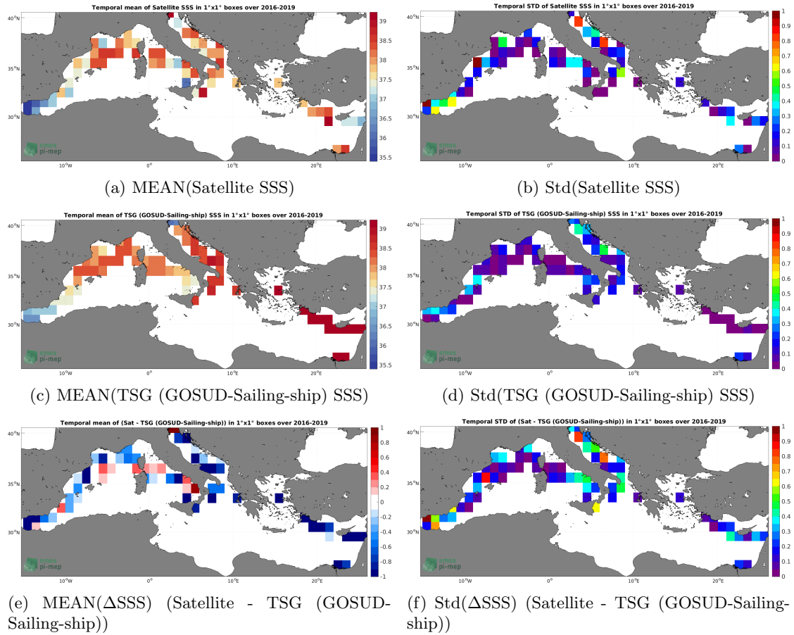
Figure 6: Temporal mean (left) and Std (right) of SSS from SMAP SSS L3 v5 - 8-Day running (RSS) (top), TSG (GOSUD-Sailing-ship) (middle), and of \Delta SSS (Satellite - TSG (GOSUD-Sailing-ship)). Only match-up pairs are used to generate these maps.
