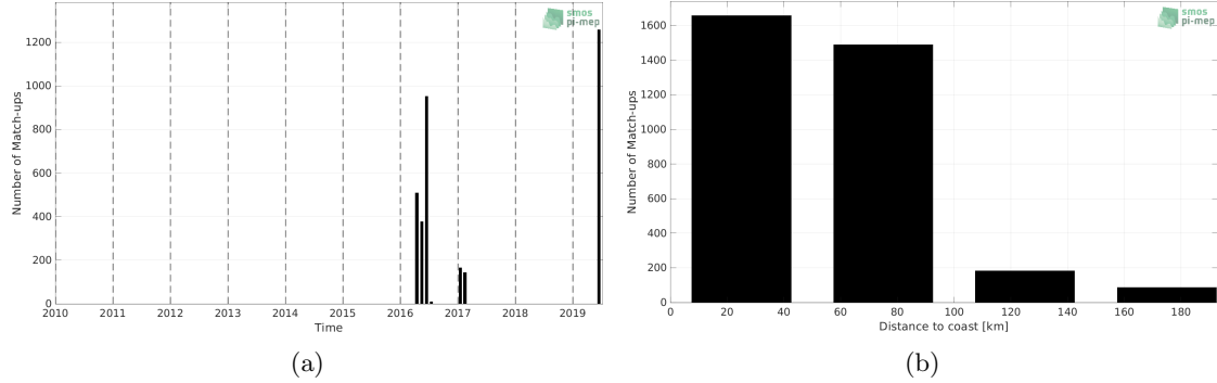
Figure 1: Number of match-ups between TSG (GOSUD-Sailing-ship) and SMAP SSS L3 v5 - 8-Day running (RSS) SSS as a function of time (a) and as function of the distance to coast (b) over the Mediterranean Sea Pi-MEP region and for the full satellite product period.
