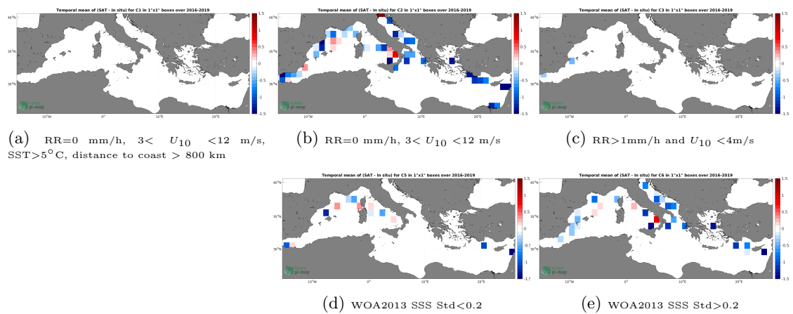
Figure 12: Temporal mean gridded over spatial boxes of size 1^\circ \times 1^\circ of \Delta SSS (SMAP SSS L3 v5 - 8-Day running (RSS) - TSG (GOSUD-Sailing-ship)) for 5 different subdatasets corresponding to: RR=0 mm/h, 3 < U_{10} < 12 m/s, SST>5°C, distance to coast > 800 km (a), RR=0 mm/h, 3 < U_{10} < 12 m/s (b), RR>1mm/h and U_{10} < 4 m/s (c), WOA2013 SSS Std<0.2 (d), WOA2013 SSS Std>0.2 (e).
