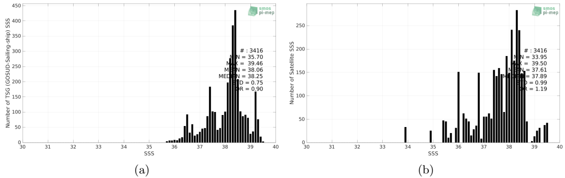
Figure 2: Histograms of SSS from TSG (GOSUD-Sailing-ship) (a) and SMAP SSS L3 v5 - 8-Day running (RSS) (b) considering all match-up pairs per bins of 0.1 over the Mediterranean Sea Pi-MEP region and for the full satellite product period.
