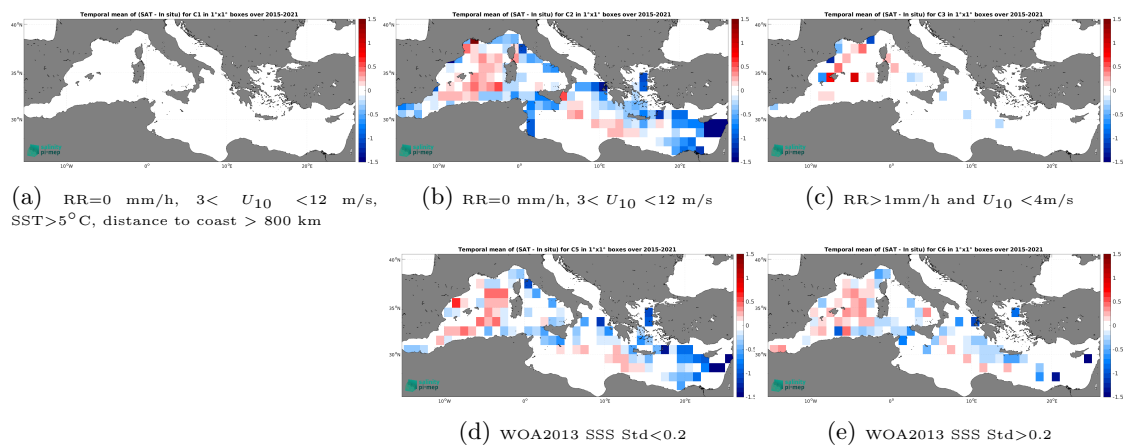
Figure 12: Temporal mean gridded over spatial boxes of size 1^\circ \times 1^\circ of \Delta\text{SSS} (SMAP SSS L3 v5 - 8-Day running (RSS) - TSG (GOSUD-Research-vessel)) for 5 different subdatasets corresponding to:RR=0 mm/h, 3 < U_{10} < 12 m/s, SST>5°C, distance to coast > 800 km (a), RR=0 mm/h, 3 < U_{10} < 12 m/s (b), RR>1mm/h and U_{10} < 4 m/s (c), WOA2013 SSS Std<0.2 (d), WOA2013 SSS Std>0.2 (e).
