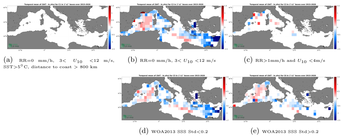
Figure 12: Temporal mean gridded over spatial boxes of size 1^\circ \times 1^\circ of \Delta SSS (SMAP SSS L3 v5 - Monthly (RSS) - TSG (GOSUD-Research-vessel)) for 5 different subdatasets corresponding to:RR=0 mm/h, 3 < U_{10} < 12 m/s, SST >5^\circ\text{C} , distance to coast > 800 km (a), RR=0 mm/h, 3 < U_{10} < 12 m/s (b), RR >1 mm/h and U_{10} < 4 m/s (c), WOA2013 SSS Std <0.2 (d), WOA2013 SSS Std >0.2 (e).
