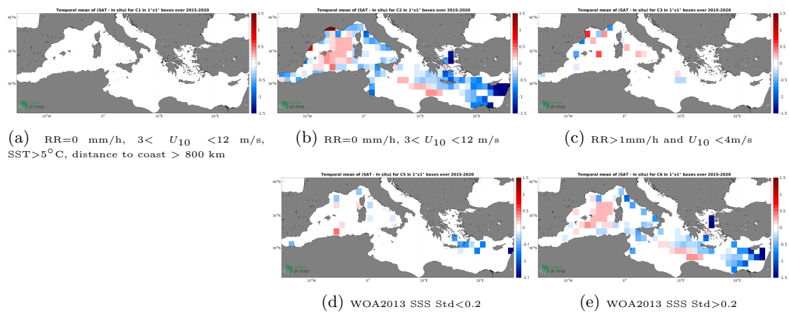
Figure 12: Temporal mean gridded over spatial boxes of size 1^\circ \times 1^\circ of \Delta\text{SSS} (SMAP SSS L3 v5 - Monthly (RSS) - TSG (GOSUD-Research-vessel)) for 5 different subdatasets corresponding to: RR=0 mm/h, 3 < U_{10} < 12 m/s, SST > 5°C, distance to coast > 800 km (a), RR=0 mm/h, 3 < U_{10} < 12 m/s (b), RR > 1 mm/h and U_{10} < 4 m/s (c), WOA2013 SSS Std < 0.2 (d), WOA2013 SSS Std > 0.2 (e).
