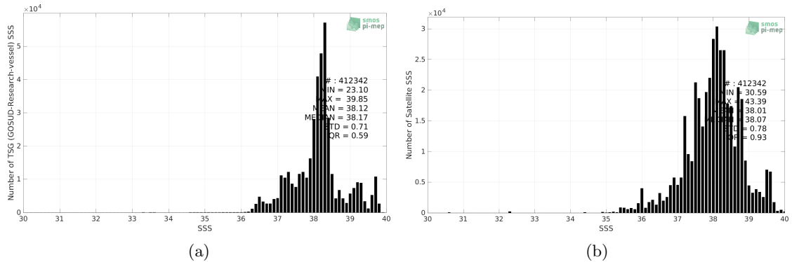
Figure 2: Histograms of SSS from TSG (GOSUD-Research-vessel) (a) and SMAP SSS L3 v5 - Monthly (RSS) (b) considering all match-up pairs per bins of 0.1 over the Mediterranean Sea Pi-MEP region and for the full satellite product period.
