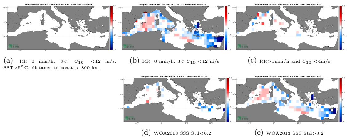
Figure 12: Temporal mean gridded over spatial boxes of size 1^\circ \times 1^\circ of \Delta\text{SSS} (SMAP SSS L3 v5 - Monthly (RSS) - TSG (GOSUD-Research-vessel)) for 5 different subdatasets corresponding to:RR=0 mm/h, 3 < U_{10} < 12 m/s, SST>5°C, distance to coast > 800 km (a), RR=0 mm/h, 3 < U_{10} < 12 m/s (b), RR>1mm/h and U_{10} < 4 m/s (c), WOA2013 SSS Std<0.2 (d), WOA2013 SSS Std>0.2 (e).
