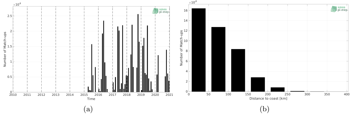
Figure 1: Number of match-ups between TSG (GOSUD-Research-vessel) and SMAP SSS L3 v5 - Monthly (RSS) SSS as a function of time (a) and as function of the distance to coast (b) over the Mediterranean Sea Pi-MEP region and for the full satellite product period.
