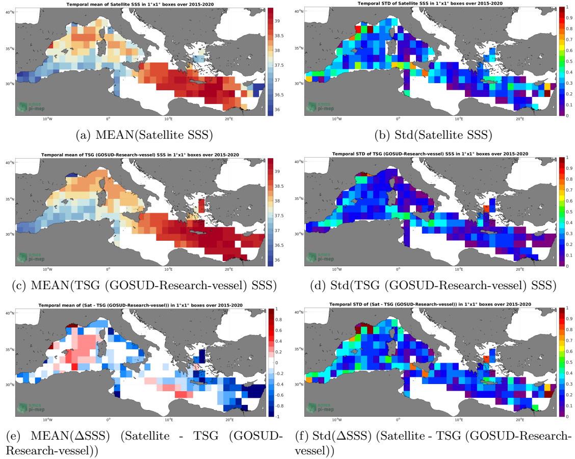
Figure 6: Temporal mean (left) and Std (right) of SSS from SMAP SSS L3 v5 - Monthly (RSS) (top), TSG (GOSUD-Research-vessel) (middle), and of \Delta SSS (Satellite - TSG (GOSUD-Research-vessel)). Only match-up pairs are used to generate these maps.
