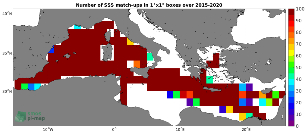
Figure 4: Number of SSS match-ups between TSG (GOSUD-Research-vessel) SSS and the SMAP SSS L3 v5 - Monthly (RSS) SSS product for the Mediterranean Sea Pi-MEP region over 1^\circ \times 1^\circ boxes and for the full satellite product period.
