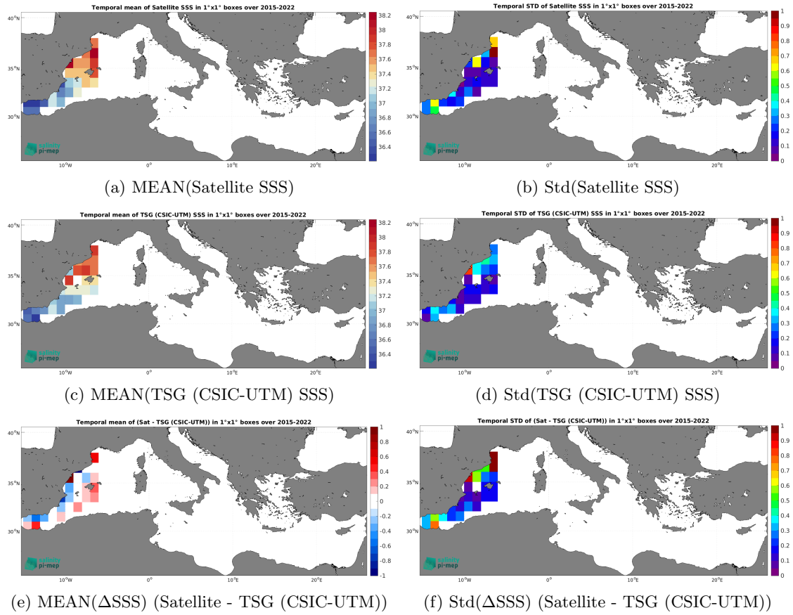
Figure 6: Temporal mean (left) and Std (right) of SSS from SMAP SSS L3 v5 - Monthly (RSS) (top), TSG (CSIC-UTM) (middle), and of \Delta SSS (Satellite - TSG (CSIC-UTM)). Only match-up pairs are used to generate these maps.
