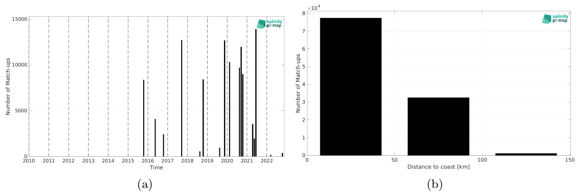
Figure 1: Number of match-ups between TSG (CSIC-UTM) and SMAP SSS L3 v5 - Monthly (RSS) SSS as a function of time (a) and as function of the distance to coast (b) over the Mediterranean Sea Pi-MEP region and for the full satellite product period.
