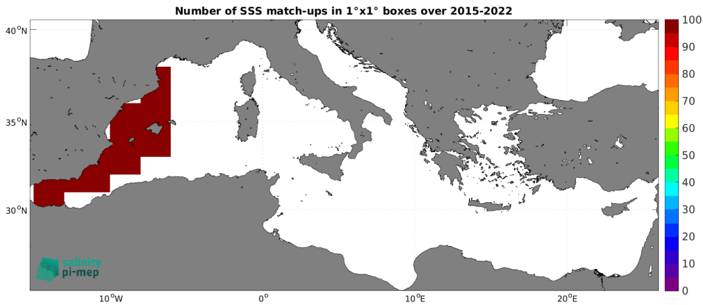
Figure 4: Number of SSS match-ups between TSG (CSIC-UTM) SSS and the SMAP SSS L3 v5 - Monthly (RSS) SSS product for the Mediterranean Sea Pi-MEP region over 1^\circ \times 1^\circ boxes and for the full satellite product period.
