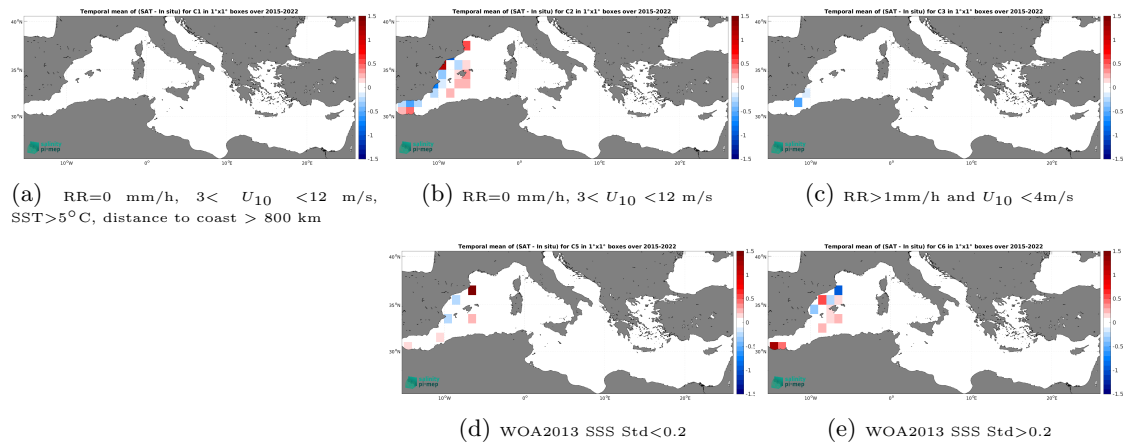
Figure 12: Temporal mean gridded over spatial boxes of size 1^\circ \times 1^\circ of \Delta SSS (SMAP SSS L3 v5 - Monthly (RSS) - TSG (CSIC-UTM)) for 5 different subdatasets corresponding to:RR=0 mm/h, 3 < U_{10} < 12 m/s, SST >5^\circ\text{C} , distance to coast > 800 km (a), RR=0 mm/h, 3 < U_{10} < 12 m/s (b), RR >1 mm/h and U_{10} < 4 m/s (c), WOA2013 SSS Std <0.2 (d), WOA2013 SSS Std >0.2 (e).
