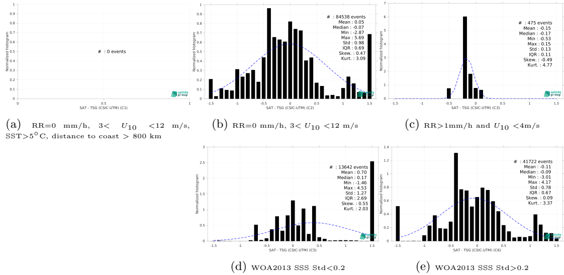
Figure 13: Normalized histogram of \Delta\text{SSS} (SMAP SSS L3 v5 - Monthly (RSS) - TSG (CSIC-UTM)) for 5 different subdatasets corresponding to: RR=0 mm/h, 3 < U_{10} < 12 m/s, SST > 5^\circ\text{C} , distance to coast > 800 km (a), RR=0 mm/h, 3 < U_{10} < 12 m/s (b), RR > 1\text{mm/h} and U_{10} < 4\text{m/s} (c), WOA2013 SSS Std < 0.2 (d), WOA2013 SSS Std > 0.2 (e).
