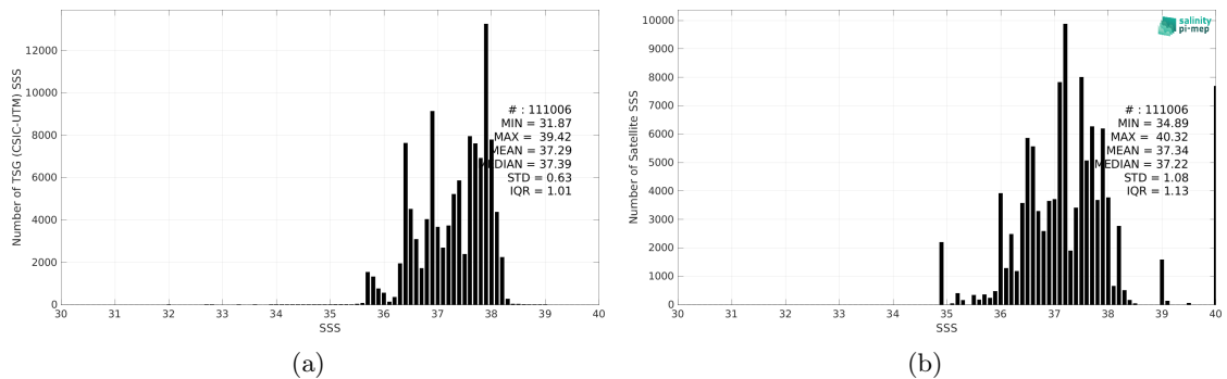
Figure 2: Histograms of SSS from TSG (CSIC-UTM) (a) and SMAP SSS L3 v5 - Monthly (RSS) (b) considering all match-up pairs per bins of 0.1 over the Mediterranean Sea Pi-MEP region and for the full satellite product period.
