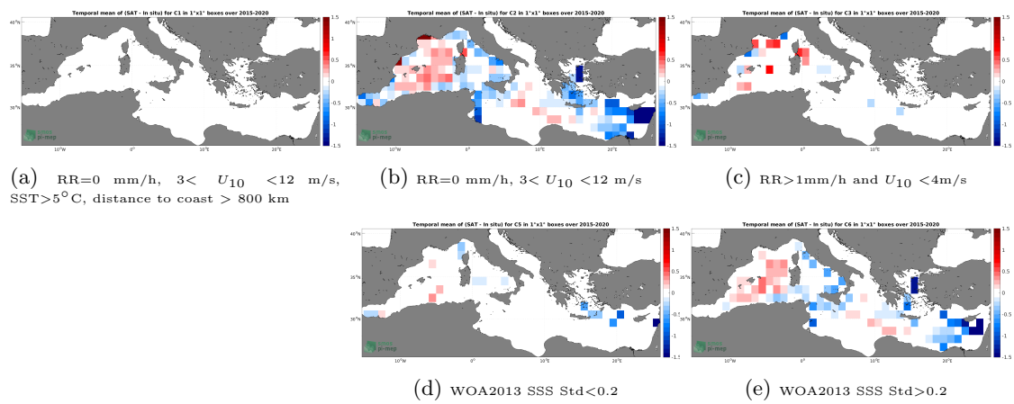
Figure 12: Temporal mean gridded over spatial boxes of size 1^\circ \times 1^\circ of \Delta\text{SSS} (SMAP SSS L3 v4 - 8-Day running (RSS) - TSG (GOSUD-Research-vessel)) for 5 different subdatasets corresponding to:RR=0 mm/h, 3 < U_{10} < 12 m/s, SST>5°C, distance to coast > 800 km (a), RR=0 mm/h, 3 < U_{10} < 12 m/s (b), RR>1mm/h and U_{10} < 4 m/s (c), WOA2013 SSS Std<0.2 (d), WOA2013 SSS Std>0.2 (e).
