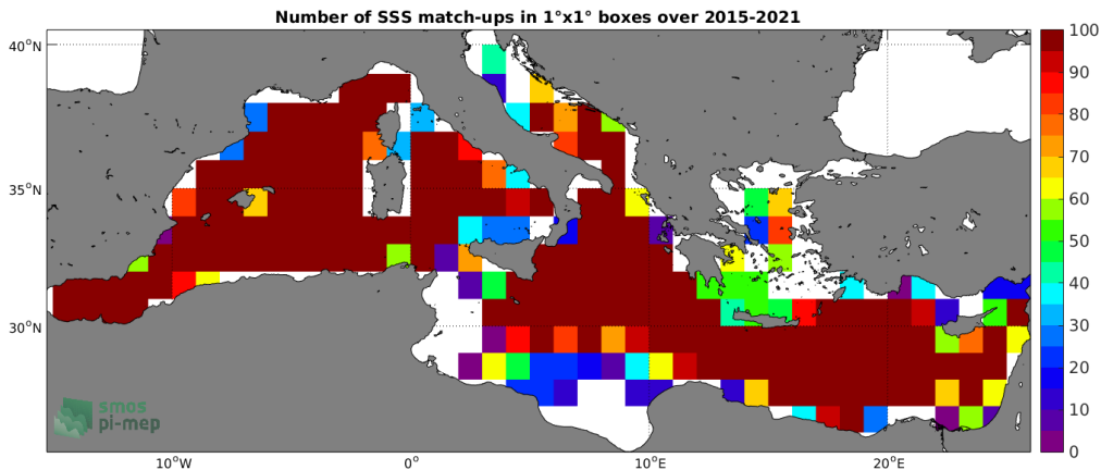
Figure 4: Number of SSS match-ups between Argo SSS and the SMAP SSS L3 v4 - 8-Day running (RSS) SSS product for the Mediterranean Sea Pi-MEP region over 1^\circ \times 1^\circ boxes and for the full satellite product period.
