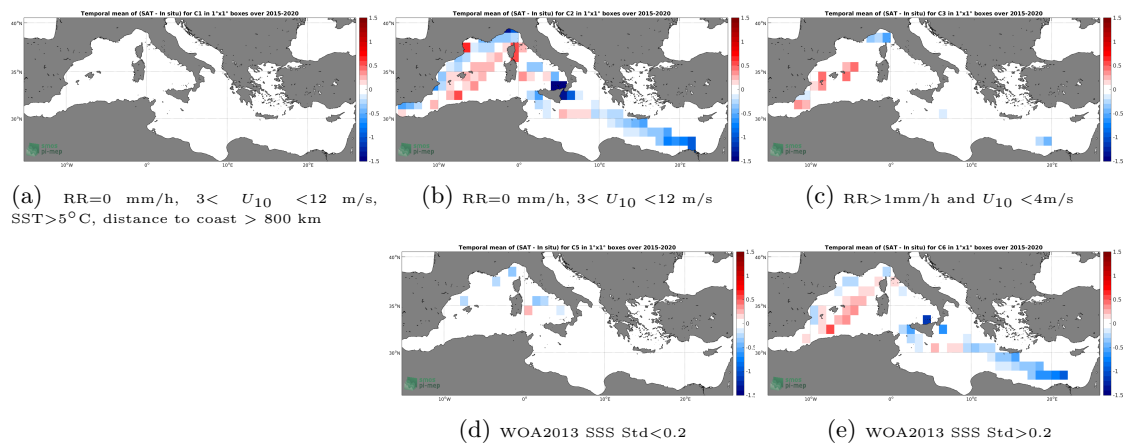
Figure 12: Temporal mean gridded over spatial boxes of size 1^\circ \times 1^\circ of \Delta\text{SSS} (SMAP SSS L3 v4 - Monthly (RSS) - TSG (LEGOS-DM)) for 5 different subdatasets corresponding to:RR=0 mm/h, 3 < U_{10} < 12 m/s, SST >5^\circ\text{C} , distance to coast > 800 km (a), RR=0 mm/h, 3 < U_{10} < 12 m/s (b), RR >1 mm/h and U_{10} < 4 m/s (c), WOA2013 SSS Std <0.2 (d), WOA2013 SSS Std >0.2 (e).
