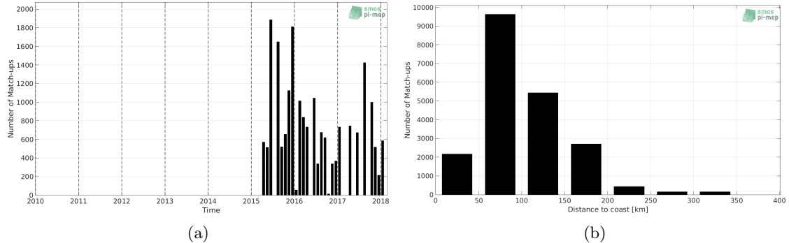
Figure 1: Number of match-ups between TSG-LEGOS-DM and SMAP-L3-RSS-V3-MONTHLY-0.25DEG-40KM SSS as a function of time (a) and as function of the distance to coast (b) over the Mediterranean Sea Pi-MEP region and for the full satellite product period.
