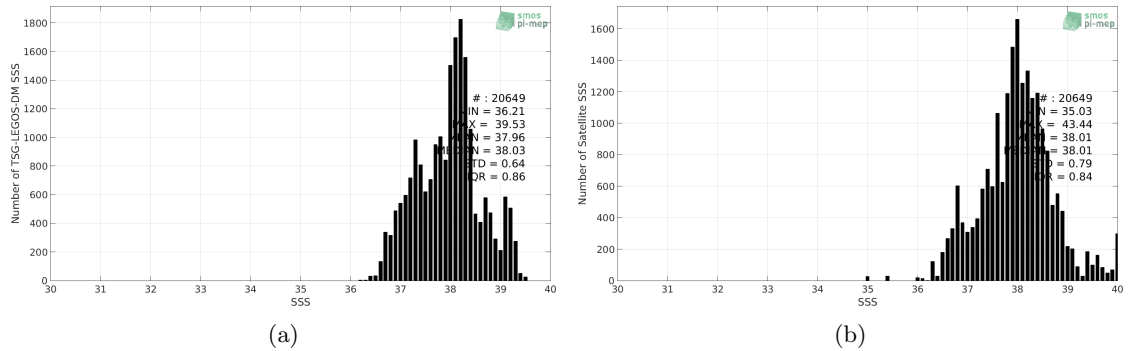
Figure 2: Histograms of SSS from TSG-LEGOS-DM (a) and SMAP-L3-RSS-V3-MONTHLY-0.25DEG-40KM (b) considering all match-up pairs per bins of 0.1 over the Mediterranean Sea Pi-MEP region and for the full satellite product period.
