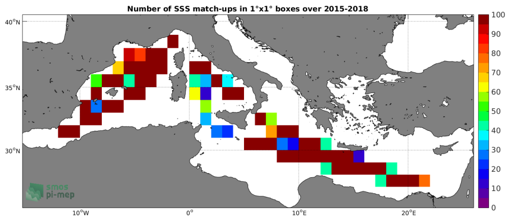
Figure 4: Number of SSS match-ups between TSG-LEGOS-DM SSS and the SMAP-L3-RSS-V3-MONTHLY-0.25DEG-40KM SSS product for the Mediterranean Sea Pi-MEP region over 1^\circ \times 1^\circ boxes and for the full satellite product period.
