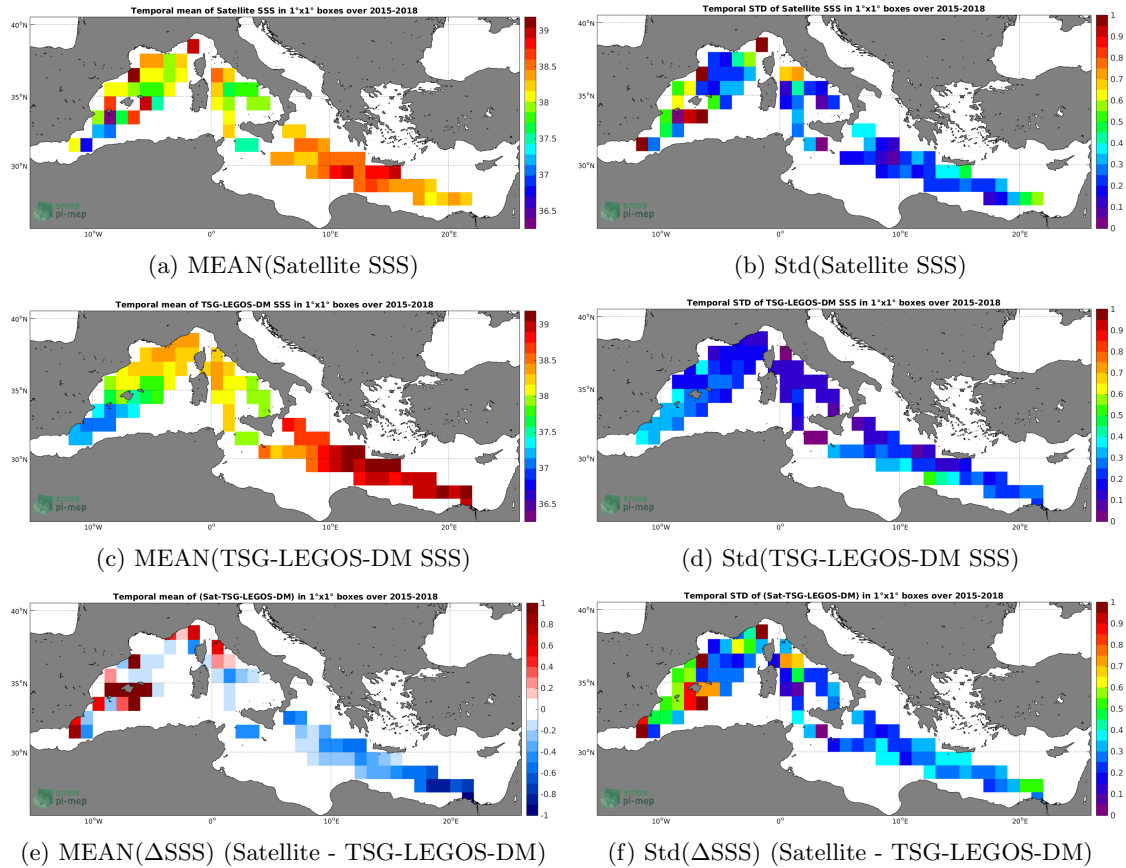
Figure 6: Temporal mean (left) and Std (right) of SSS from SMAP-L3-RSS-V3-MONTHLY-0.25DEG-40KM (top), TSG-LEGOS-DM (middle), and of \Delta SSS (Satellite - TSG-LEGOS-DM). Only match-up pairs are used to generate these maps.
