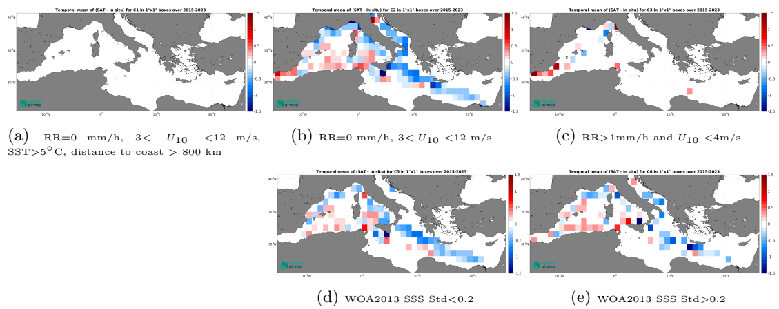
Figure 14: Temporal mean gridded over spatial boxes of size 1^\circ \times 1^\circ of \Delta SSS (SMAP SSS L3 v5.0 - 8-Day running (JPL) - TSG (LEGOS-DM)) for 5 different subdatasets corresponding to:RR=0 mm/h, 3 < U_{10} < 12 m/s, SST>5°C, distance to coast > 800 km (a), RR=0 mm/h, 3 < U_{10} < 12 m/s (b), RR>1mm/h and U_{10} < 4 m/s (c), WOA2013 SSS Std<0.2 (d), WOA2013 SSS Std>0.2 (e).
