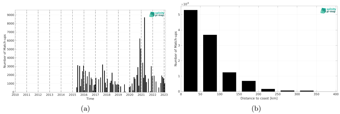
Figure 2: Number of match-ups between TSG (LEGOS-DM) and SMAP SSS L3 v5.0 - 8-Day running (JPL) SSS as a function of time (a) and as function of the distance to coast (b) over the Mediterranean Sea Pi-MEP region and for the full satellite product period.
