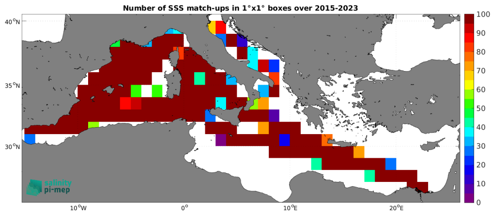
Figure 5: Number of SSS match-ups between TSG (LEGOS-DM) SSS and the SMAP SSS L3 v5.0 - 8-Day running (JPL) SSS product for the Mediterranean Sea Pi-MEP region over 1^\circ \times 1^\circ boxes and for the full satellite product period.
