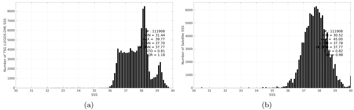
Figure 3: Histograms of SSS from TSG (LEGOS-DM) (a) and SMAP SSS L3 v5.0 - 8-Day running (JPL) (b) considering all match-up pairs per bins of 0.1 over the Mediterranean Sea Pi-MEP region and for the full satellite product period.
