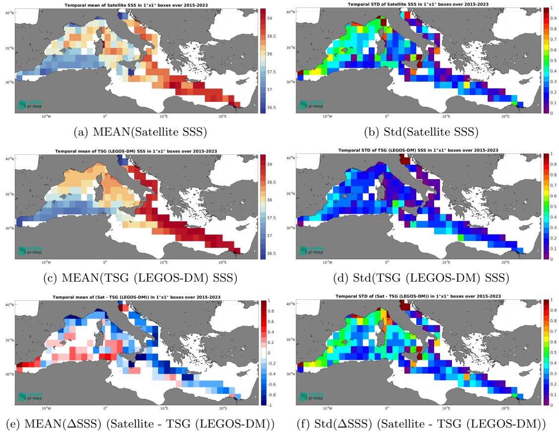
Figure 7: Temporal mean (left) and Std (right) of SSS from SMAP SSS L3 v5.0 - 8-Day running (JPL) (top), TSG (LEGOS-DM) (middle), and of \Delta SSS (Satellite - TSG (LEGOS-DM)). Only match-up pairs are used to generate these maps.
