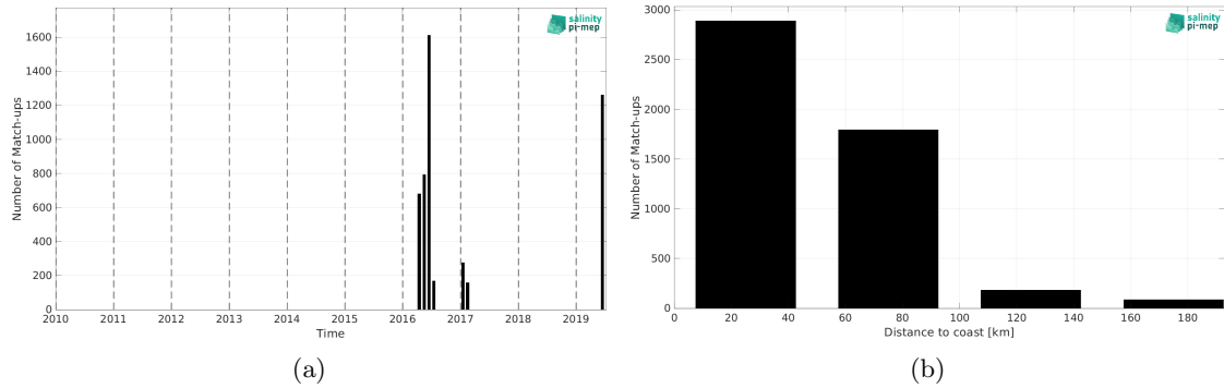
Figure 2: Number of match-ups between TSG (GOSUD-Sailing-ship) and SMAP SSS L3 v5.0 - 8-Day running (JPL) SSS as a function of time (a) and as function of the distance to coast (b) over the Mediterranean Sea Pi-MEP region and for the full satellite product period.
