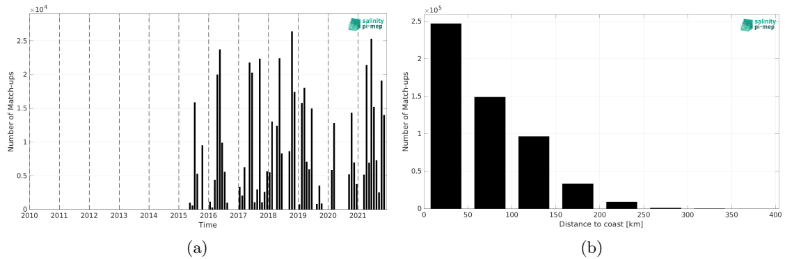
Figure 2: Number of match-ups between TSG (GOSUD-Research-vessel) and SMAP SSS L3 v5.0 - 8-Day running (JPL) SSS as a function of time (a) and as function of the distance to coast (b) over the Mediterranean Sea Pi-MEP region and for the full satellite product period.
