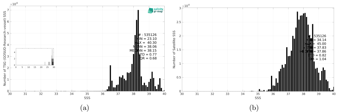
Figure 3: Histograms of SSS from TSG (GOSUD-Research-vessel) (a) and SMAP SSS L3 v5.0 - 8-Day running (JPL) (b) considering all match-up pairs per bins of 0.1 over the Mediterranean Sea Pi-MEP region and for the full satellite product period.
