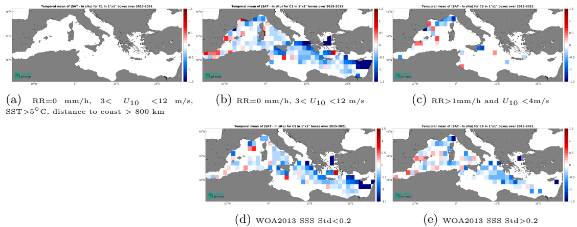
Figure 14: Temporal mean gridded over spatial boxes of size 1^\circ \times 1^\circ of \Delta\text{SSS} (SMAP SSS L3 v5.0 - 8-Day running (JPL) - TSG (GOSUD-Research-vessel)) for 5 different subdatasets corresponding to:RR=0 mm/h, 3 < U_{10} < 12 m/s, SST>5°C, distance to coast > 800 km (a), RR=0 mm/h, 3 < U_{10} < 12 m/s (b), RR>1mm/h and U_{10} < 4 m/s (c), WOA2013 SSS Std<0.2 (d), WOA2013 SSS Std>0.2 (e).
