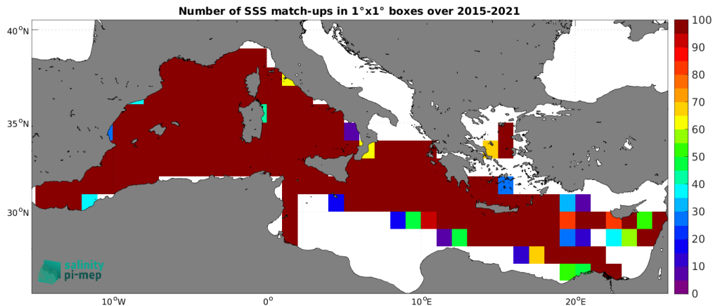
Figure 5: Number of SSS match-ups between TSG (GOSUD-Research-vessel) SSS and the SMAP SSS L3 v5.0 - 8-Day running (JPL) SSS product for the Mediterranean Sea Pi-MEP region over 1^\circ \times 1^\circ boxes and for the full satellite product period.
