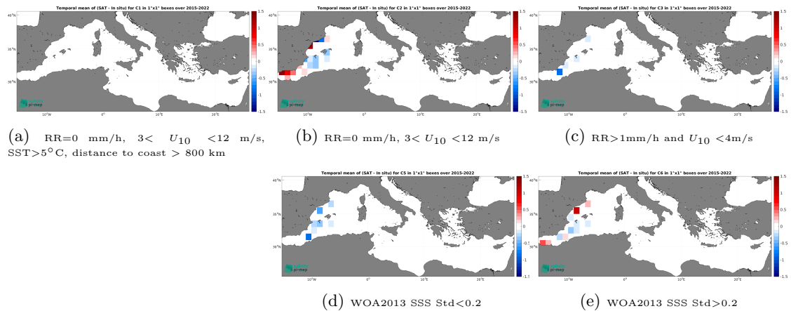
Figure 12: Temporal mean gridded over spatial boxes of size 1^\circ \times 1^\circ of \Delta SSS (SMAP SSS L3 v5.0 - 8-Day running (JPL) - TSG (CSIC-UTM)) for 5 different subdatasets corresponding to:RR=0 mm/h, 3 < U_{10} < 12 m/s, SST >5^\circ\text{C} , distance to coast > 800 km (a), RR=0 mm/h, 3 < U_{10} < 12 m/s (b), RR >1 mm/h and U_{10} < 4 m/s (c), WOA2013 SSS Std <0.2 (d), WOA2013 SSS Std >0.2 (e).
