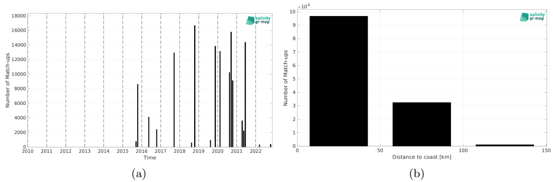
Figure 1: Number of match-ups between TSG (CSIC-UTM) and SMAP SSS L3 v5.0 - 8-Day running (JPL) SSS as a function of time (a) and as function of the distance to coast (b) over the Mediterranean Sea Pi-MEP region and for the full satellite product period.
