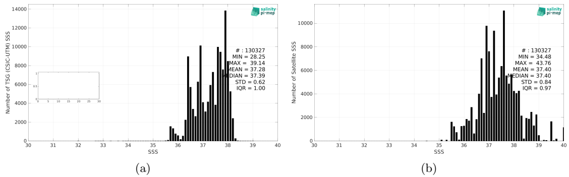
Figure 2: Histograms of SSS from TSG (CSIC-UTM) (a) and SMAP SSS L3 v5.0 - 8-Day running (JPL) (b) considering all match-up pairs per bins of 0.1 over the Mediterranean Sea Pi-MEP region and for the full satellite product period.
