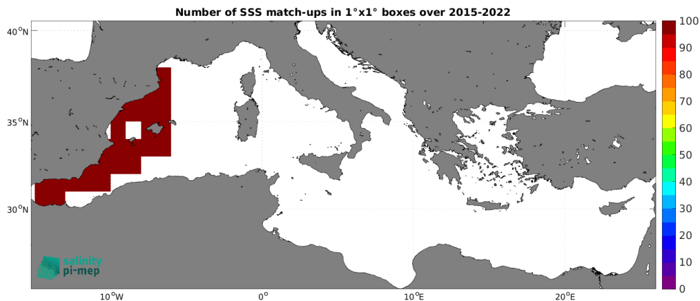
Figure 4: Number of SSS match-ups between TSG (CSIC-UTM) SSS and the SMAP SSS L3 v5.0 - 8-Day running (JPL) SSS product for the Mediterranean Sea Pi-MEP region over 1^\circ \times 1^\circ boxes and for the full satellite product period.
