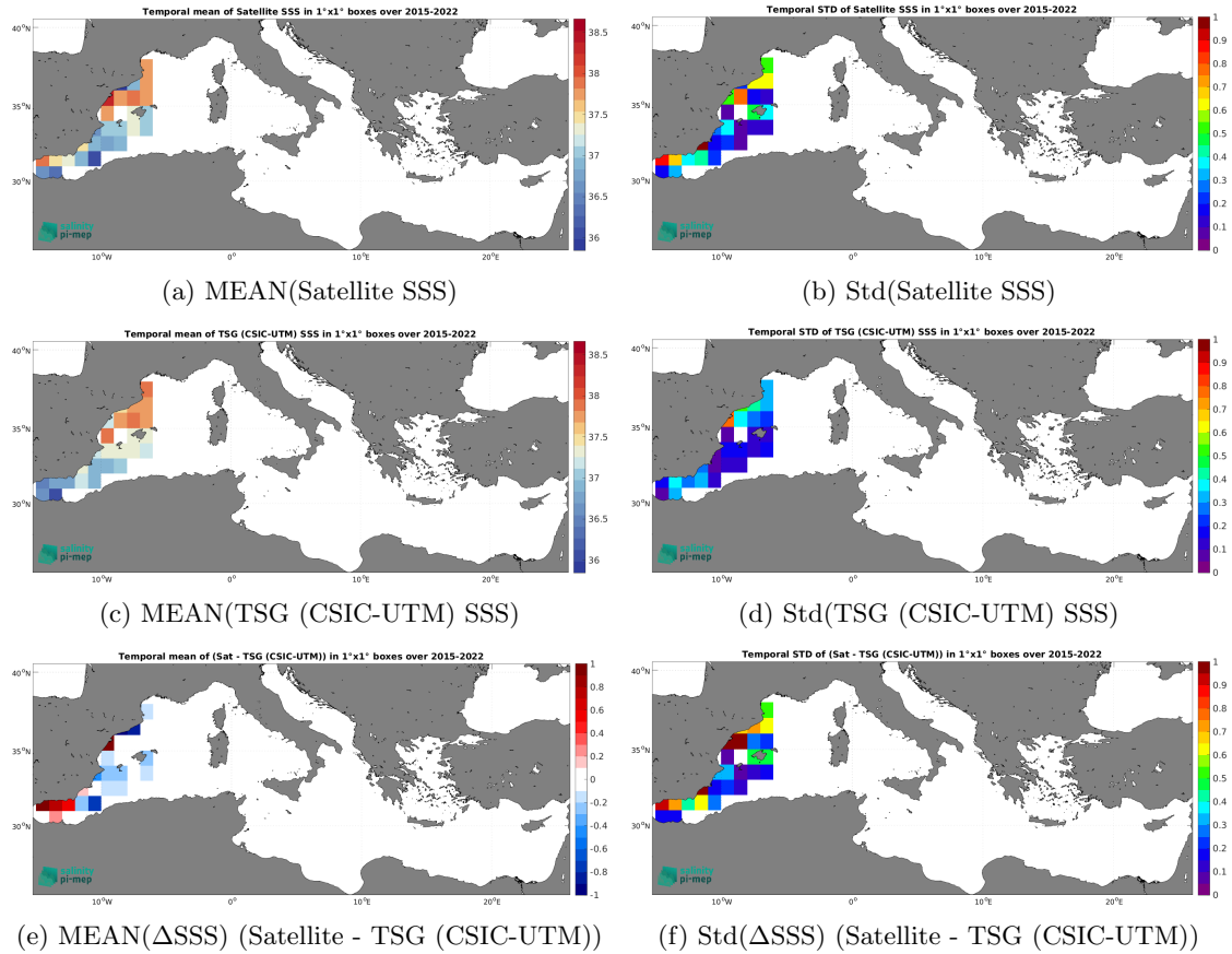
Figure 6: Temporal mean (left) and Std (right) of SSS from SMAP SSS L3 v5.0 - 8-Day running (JPL) (top), TSG (CSIC-UTM) (middle), and of \Delta SSS (Satellite - TSG (CSIC-UTM)). Only match-up pairs are used to generate these maps.
