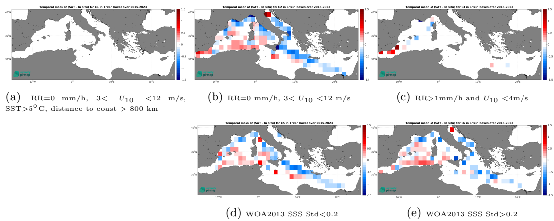
Figure 14: Temporal mean gridded over spatial boxes of size 1^\circ \times 1^\circ of \Delta\text{SSS} (SMAP SSS L3 v5.0 - Monthly (JPL) - TSG (LEGOS-DM)) for 5 different subdatasets corresponding to:RR=0 mm/h, 3 < U_{10} < 12 m/s, SST >5^\circ\text{C} , distance to coast > 800 km (a), RR=0 mm/h, 3 < U_{10} < 12 m/s (b), RR >1 mm/h and U_{10} < 4 m/s (c), WOA2013 SSS Std <0.2 (d), WOA2013 SSS Std >0.2 (e).
