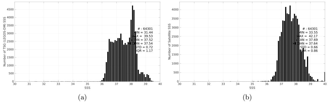
Figure 3: Histograms of SSS from TSG (LEGOS-DM) (a) and SMAP SSS L3 v5.0 - Monthly (JPL) (b) considering all match-up pairs per bins of 0.1 over the Mediterranean Sea Pi-MEP region and for the full satellite product period.
