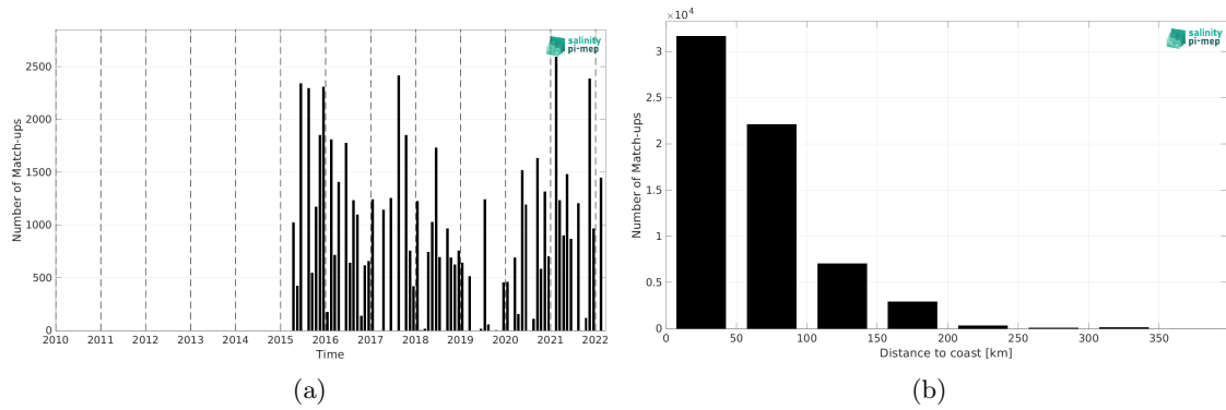
Figure 2: Number of match-ups between TSG (LEGOS-DM) and SMAP SSS L3 v5.0 - Monthly (JPL) SSS as a function of time (a) and as function of the distance to coast (b) over the Mediterranean Sea Pi-MEP region and for the full satellite product period.
