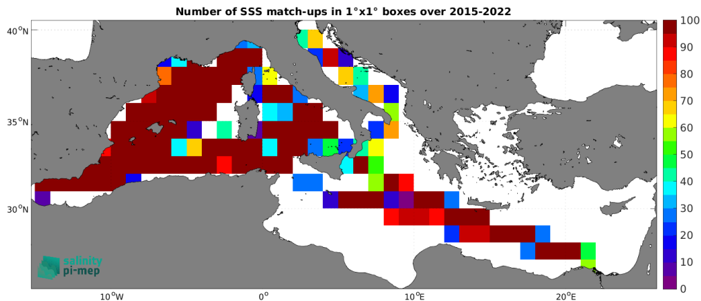
Figure 5: Number of SSS match-ups between TSG (LEGOS-DM) SSS and the SMAP SSS L3 v5.0 - Monthly (JPL) SSS product for the Mediterranean Sea Pi-MEP region over 1^\circ \times 1^\circ boxes and for the full satellite product period.
