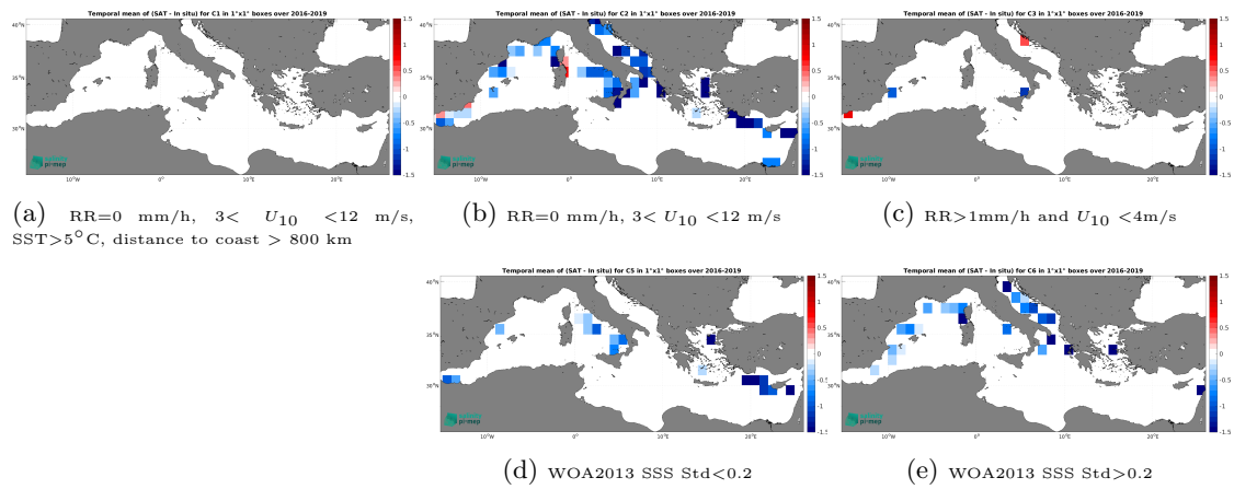
Figure 12: Temporal mean gridded over spatial boxes of size 1^\circ \times 1^\circ of \Delta SSS (SMAP SSS L3 v5.0 - Monthly (JPL) - TSG (GOSUD-Sailing-ship)) for 5 different subdatasets corresponding to:RR=0 mm/h, 3 < U_{10} < 12 m/s, SST >5^\circ\text{C} , distance to coast > 800 km (a), RR=0 mm/h, 3 < U_{10} < 12 m/s (b), RR >1 mm/h and U_{10} < 4 m/s (c), WOA2013 SSS Std <0.2 (d), WOA2013 SSS Std >0.2 (e).
