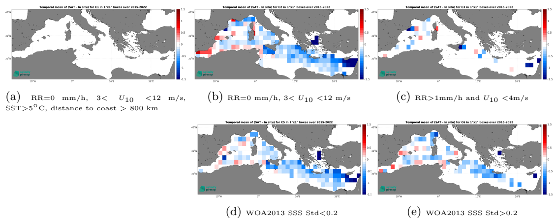
Figure 14: Temporal mean gridded over spatial boxes of size 1^\circ \times 1^\circ of \Delta SSS (SMAP SSS L3 v5.0 - Monthly (JPL) - TSG (GOSUD-Research-vessel)) for 5 different subdatasets corresponding to:RR=0 mm/h, 3 < U_{10} < 12 m/s, SST >5^\circ\text{C} , distance to coast > 800 km (a), RR=0 mm/h, 3 < U_{10} < 12 m/s (b), RR >1 mm/h and U_{10} < 4 m/s (c), WOA2013 SSS Std <0.2 (d), WOA2013 SSS Std >0.2 (e).
