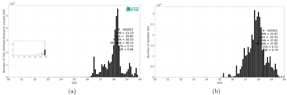
Figure 3: Histograms of SSS from TSG (GOSUD-Research-vessel) (a) and SMAP SSS L3 v5.0 - Monthly (JPL) (b) considering all match-up pairs per bins of 0.1 over the Mediterranean Sea Pi-MEP region and for the full satellite product period.
