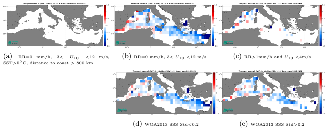
Figure 14: Temporal mean gridded over spatial boxes of size 1^\circ \times 1^\circ of \Delta SSS (SMAP SSS L3 v5.0 - Monthly (JPL) - TSG (GOSUD-Research-vessel)) for 5 different subdatasets corresponding to:RR=0 mm/h, 3 < U_{10} < 12 m/s, SST >5^\circ C, distance to coast > 800 km (a), RR=0 mm/h, 3 < U_{10} < 12 m/s (b), RR >1 mm/h and U_{10} < 4 m/s (c), WOA2013 SSS Std <0.2 (d), WOA2013 SSS Std >0.2 (e).
