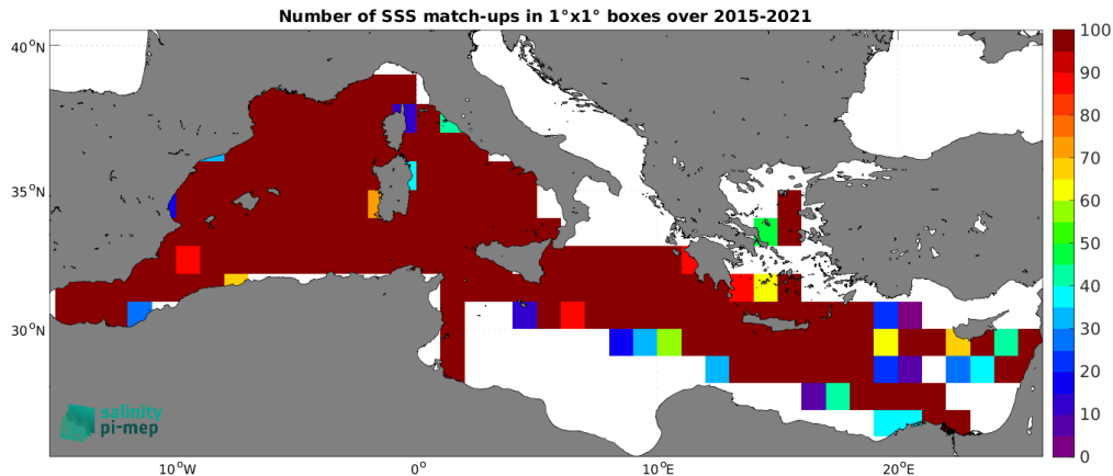
Figure 5: Number of SSS match-ups between TSG (GOSUD-Research-vessel) SSS and the SMAP SSS L3 v5.0 - Monthly (JPL) SSS product for the Mediterranean Sea Pi-MEP region over 1^\circ \times 1^\circ boxes and for the full satellite product period.
