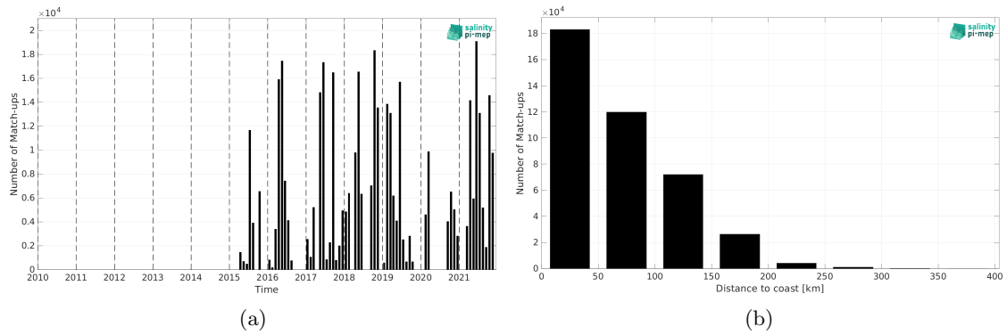
Figure 2: Number of match-ups between TSG (GOSUD-Research-vessel) and SMAP SSS L3 v5.0 - Monthly (JPL) SSS as a function of time (a) and as function of the distance to coast (b) over the Mediterranean Sea Pi-MEP region and for the full satellite product period.
