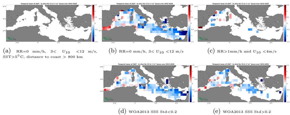
Figure 12: Temporal mean gridded over spatial boxes of size 1^\circ \times 1^\circ of \Delta SSS (SMAP SSS L3 v5.0 - Monthly (JPL) - TSG (GOSUD-Research-vessel)) for 5 different subdatasets corresponding to:RR=0 mm/h, 3 < U_{10} < 12 m/s, SST >5^\circ\text{C} , distance to coast > 800 km (a), RR=0 mm/h, 3 < U_{10} < 12 m/s (b), RR >1 mm/h and U_{10} < 4 m/s (c), WOA2013 SSS Std <0.2 (d), WOA2013 SSS Std >0.2 (e).
