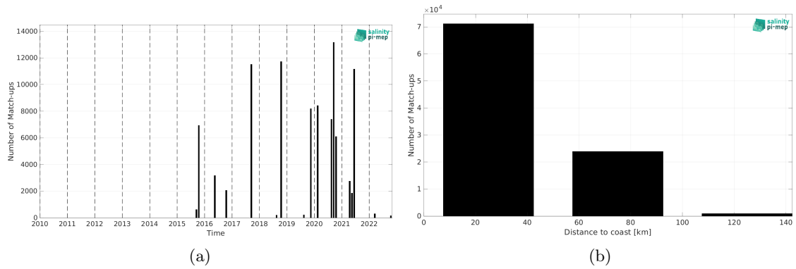
Figure 2: Number of match-ups between TSG (CSIC-UTM) and SMAP SSS L3 v5.0 - Monthly (JPL) SSS as a function of time (a) and as function of the distance to coast (b) over the Mediterranean Sea Pi-MEP region and for the full satellite product period.
