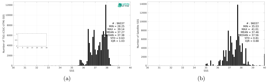
Figure 3: Histograms of SSS from TSG (CSIC-UTM) (a) and SMAP SSS L3 v5.0 - Monthly (JPL) (b) considering all match-up pairs per bins of 0.1 over the Mediterranean Sea Pi-MEP region and for the full satellite product period.
