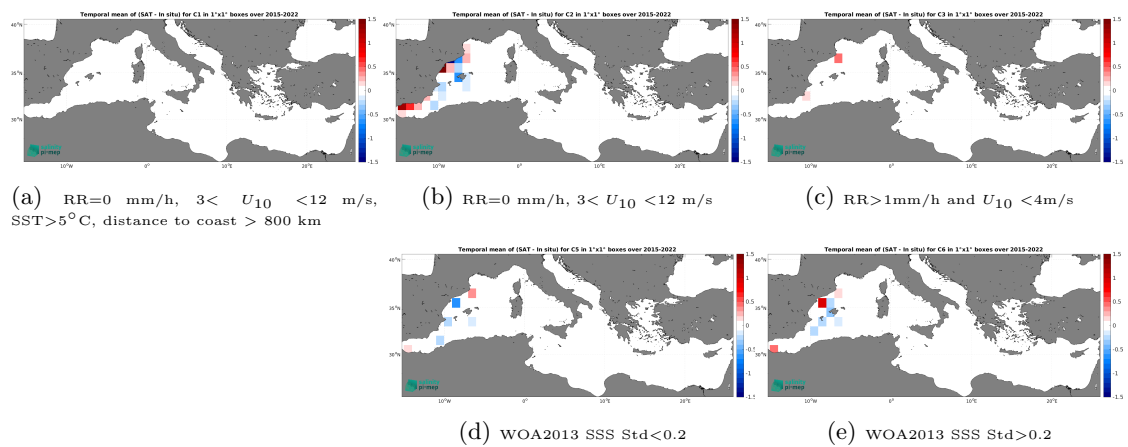
Figure 14: Temporal mean gridded over spatial boxes of size 1^\circ \times 1^\circ of \Delta SSS (SMAP SSS L3 v5.0 - Monthly (JPL) - TSG (CSIC-UTM)) for 5 different subdatasets corresponding to:RR=0 mm/h, 3 < U_{10} < 12 m/s, SST >5^\circ\text{C} , distance to coast > 800 km (a), RR=0 mm/h, 3 < U_{10} < 12 m/s (b), RR >1 mm/h and U_{10} < 4 m/s (c), WOA2013 SSS Std <0.2 (d), WOA2013 SSS Std >0.2 (e).
