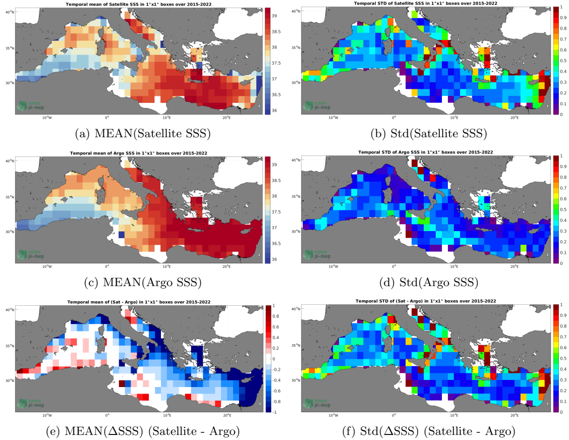
Figure 6: Temporal mean (left) and Std (right) of SSS from SMAP SSS L3 v5.0 - Monthly (JPL) (top), Argo (middle), and of \Delta\text{SSS} (Satellite - Argo). Only match-up pairs are used to generate these maps.
