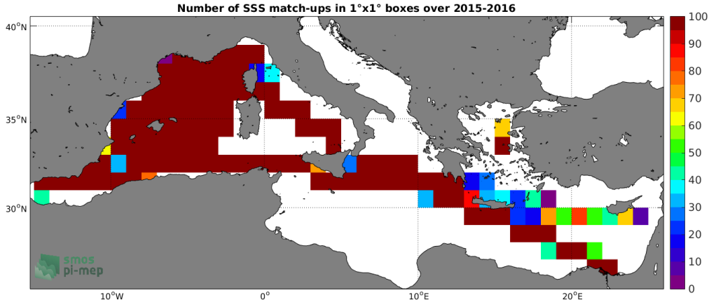
Figure 4: Number of SSS match-ups between TSG-GOSUD-Research-vessel SSS and the SMAP-L3-JPL-V4-8DAY-RUNNING-60KM SSS product for the Mediterranean Sea Pi-MEP region over 1^\circ \times 1^\circ boxes and for the full satellite product period.
