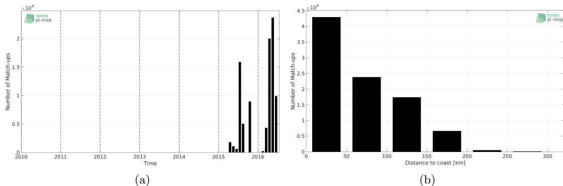
Figure 1: Number of match-ups between TSG-GOSUD-Research-vessel and SMAP-L3-JPL-V4-8DAY-RUNNING-60KM SSS as a function of time (a) and as function of the distance to coast (b) over the Mediterranean Sea Pi-MEP region and for the full satellite product period.
