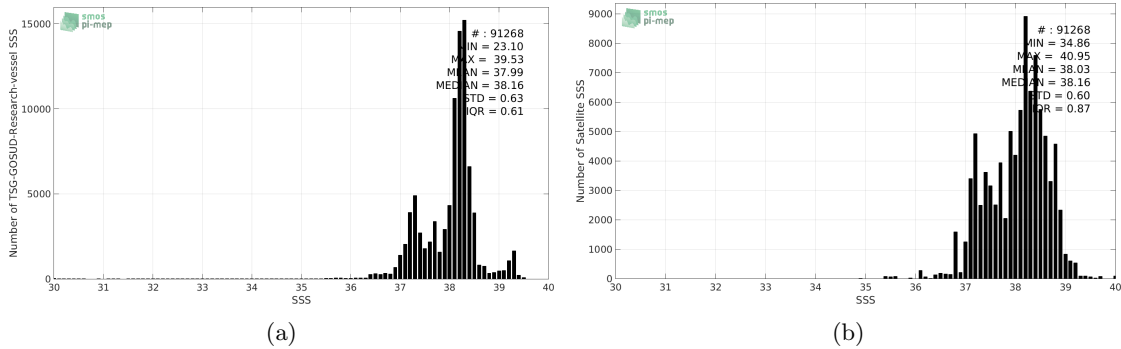
Figure 2: Histograms of SSS from TSG-GOSUD-Research-vessel (a) and SMAP-L3-JPL-V4-8DAY-RUNNING-60KM (b) considering all match-up pairs per bins of 0.1 over the Mediterranean Sea Pi-MEP region and for the full satellite product period.
