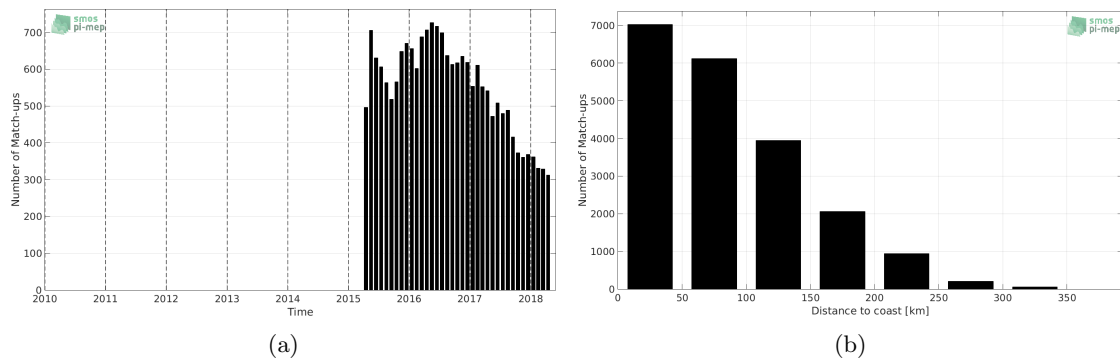
Figure 1: Number of match-ups between Argo and SMAP-L3-JPL-V4-MONTHLY-60KM SSS as a function of time (a) and as function of the distance to coast (b) over the Mediterranean Sea Pi-MEP region and for the full satellite product period.
