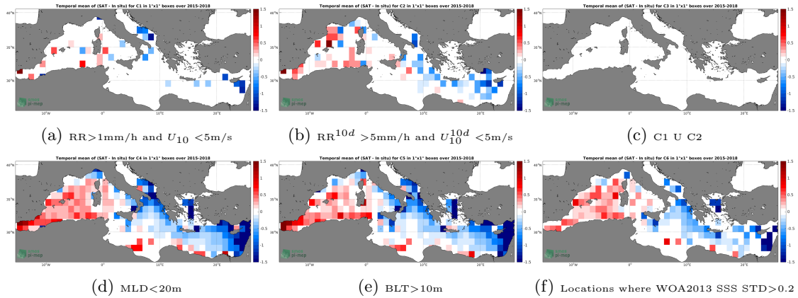
Figure 12: Temporal mean gridded over spatial boxes of size 1^\circ \times 1^\circ of \Delta\text{SSS} (SMAP-L3-JPL-V4-MONTHLY-60KM - Argo) for 6 different subdatasets corresponding to: \text{RR} > 1\text{mm/h} and U_{10} < 5\text{m/s} (a), \text{RR}^{10d} > 5\text{mm/h} and U_{10}^{10d} < 5\text{m/s} (b), C1 U C2 (c), \text{MLD} < 20\text{m} (d), \text{BLT} > 10\text{m} (e), Locations where WOA2013 SSS STD > 0.2 (f).
