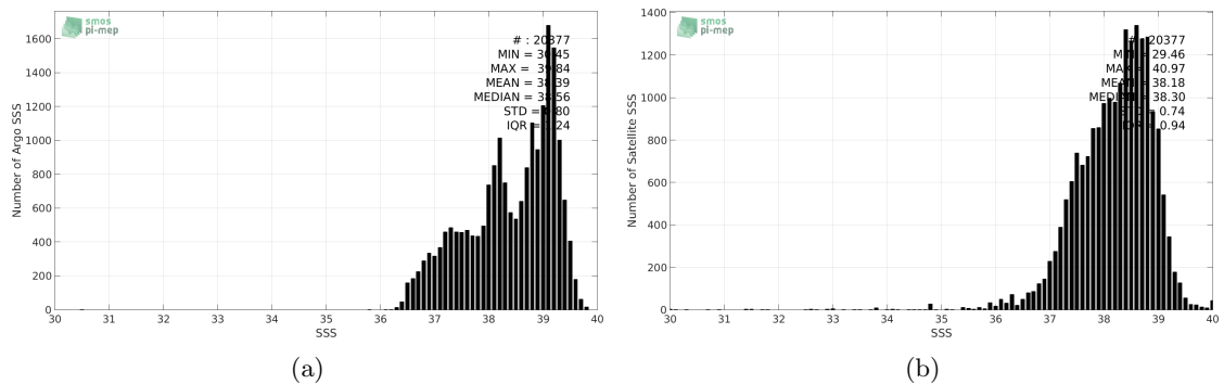
Figure 2: Histograms of SSS from Argo (a) and SMAP-L3-JPL-V4-MONTHLY-60KM (b) considering all match-up pairs per bins of 0.1 over the Mediterranean Sea Pi-MEP region and for the full satellite product period.
