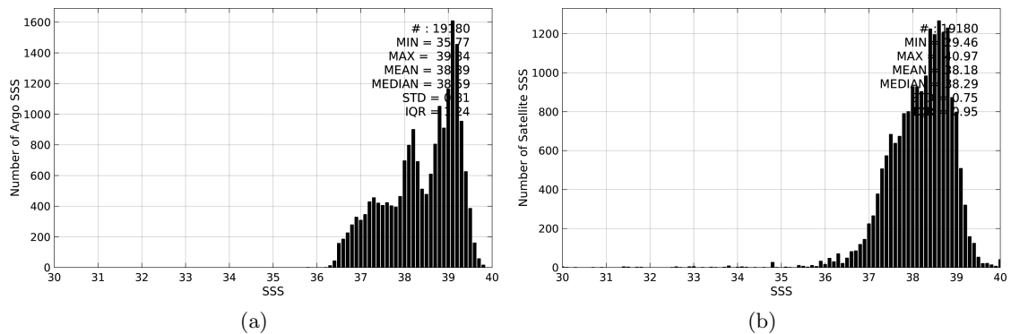
Figure 2: Histograms of SSS from Argo (a) and SMAP-L3-JPL-V4-MONTHLY-60KM (b) considering all match-up pairs per bins of 0.1 over the Mediterranean Sea Pi-MEP region and for the full satellite product period.
