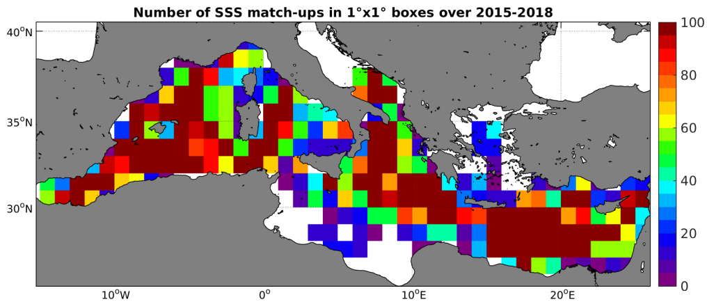
Figure 4: Number of SSS match-ups between Argo SSS and the SMAP-L3-JPL-V4-MONTHLY-60KM SSS product for the Mediterranean Sea Pi-MEP region over 1^\circ \times 1^\circ boxes and for the full satellite product period.
