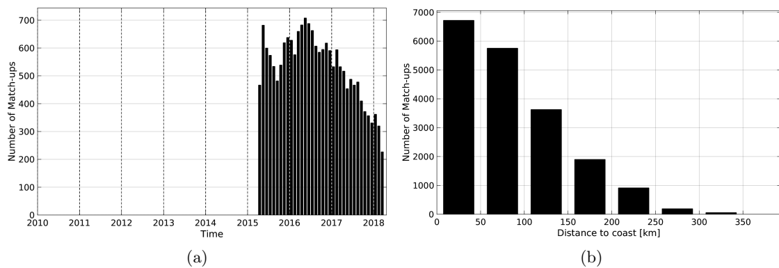
Figure 1: Number of match-ups between Argo and SMAP-L3-JPL-V4-MONTHLY-60KM SSS as a function of time (a) and as function of the distance to coast (b) over the Mediterranean Sea Pi-MEP region and for the full satellite product period.
