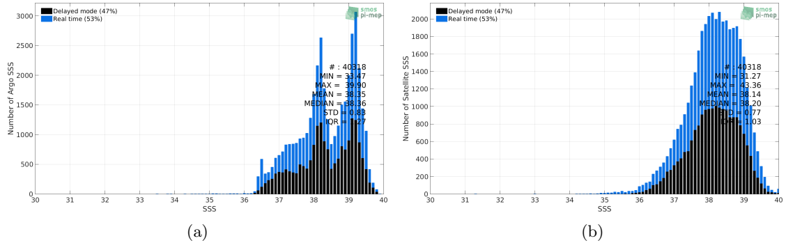
Figure 2: Histograms of SSS from Argo (a) and SMAP SSS L2-AVERAGED v5 (RSS) (b) considering all match-up pairs per bins of 0.1 over the Mediterranean Sea Pi-MEP region and for the full satellite product period.
