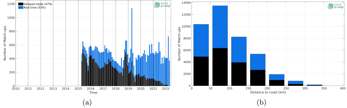
Figure 1: Number of match-ups between Argo and SMAP SSS L2-AVERAGED v5 (RSS) SSS as a function of time (a) and as function of the distance to coast (b) over the Mediterranean Sea Pi-MEP region and for the full satellite product period.
