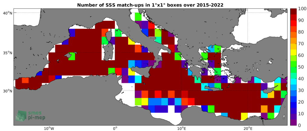
Figure 4: Number of SSS match-ups between Argo SSS and the SMAP SSS L2-AVERAGED v5 (RSS) SSS product for the Mediterranean Sea Pi-MEP region over 1^\circ \times 1^\circ boxes and for the full satellite product period.
