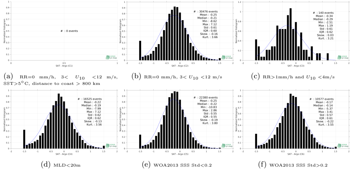
Figure 13: Normalized histogram of \Delta\text{SSS} (SMAP SSS L2-AVERAGED v5.0 (JPL) - Argo) for 6 different subdatasets corresponding to: RR=0 mm/h, 3 < U_{10} < 12 m/s, SST>5°C, distance to coast > 800 km (a), RR=0 mm/h, 3 < U_{10} < 12 m/s (b), RR>1mm/h and U_{10} < 4 m/s (c), MLD<20m (d), WOA2013 SSS Std<0.2 (e), WOA2013 SSS Std>0.2 (f).
