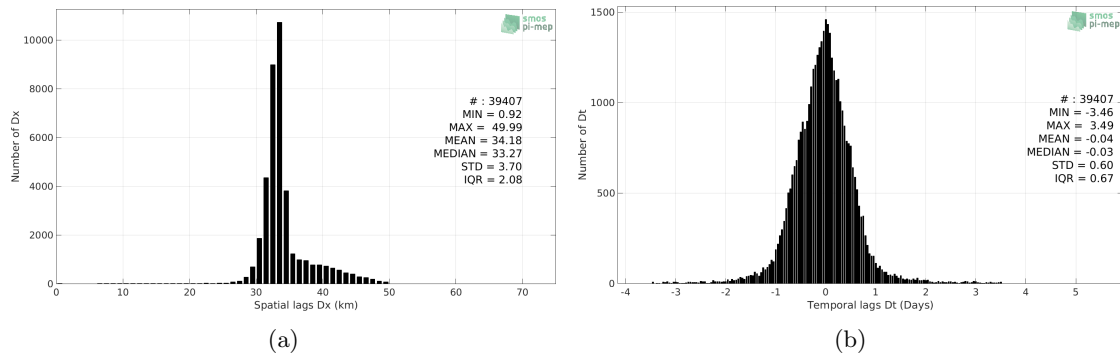
Figure 5: Histograms of the spatial (a) and temporal (b) lags between the location/time of the Argo measurement and the date of the corresponding SMAP SSS L2-AVERAGED v5.0 (JPL) SSS pixel.
