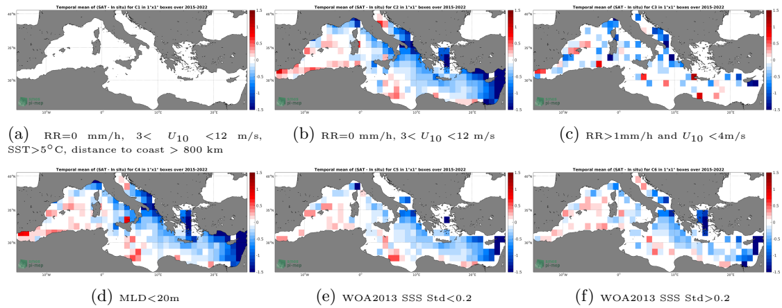
Figure 12: Temporal mean gridded over spatial boxes of size 1^\circ \times 1^\circ of \Delta SSS (SMAP SSS L2-AVERAGED v5.0 (JPL) - Argo) for 6 different subdatasets corresponding to:RR=0 mm/h, 3 < U_{10} < 12 m/s, SST >5^\circ C, distance to coast > 800 km (a), RR=0 mm/h, 3 < U_{10} < 12 m/s (b), RR >1 mm/h and U_{10} < 4 m/s (c),MLD <20 m (d),WOA2013 SSS Std <0.2 (e),WOA2013 SSS Std >0.2 (f).
