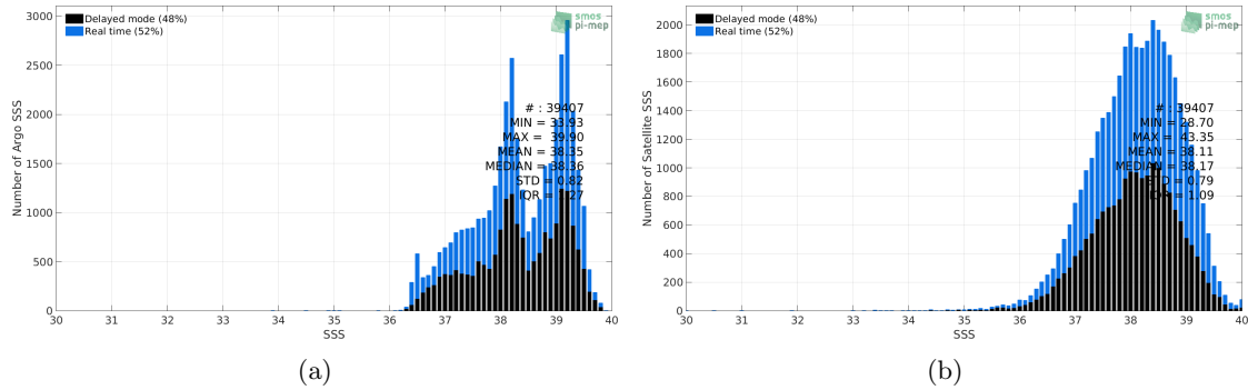
Figure 2: Histograms of SSS from Argo (a) and SMAP SSS L2-AVERAGED v5.0 (JPL) (b) considering all match-up pairs per bins of 0.1 over the Mediterranean Sea Pi-MEP region and for the full satellite product period.
