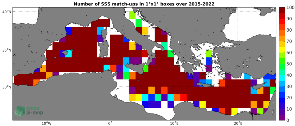
Figure 4: Number of SSS match-ups between Argo SSS and the SMAP SSS L2-AVERAGED v5.0 (JPL) SSS product for the Mediterranean Sea Pi-MEP region over 1^\circ \times 1^\circ boxes and for the full satellite product period.
