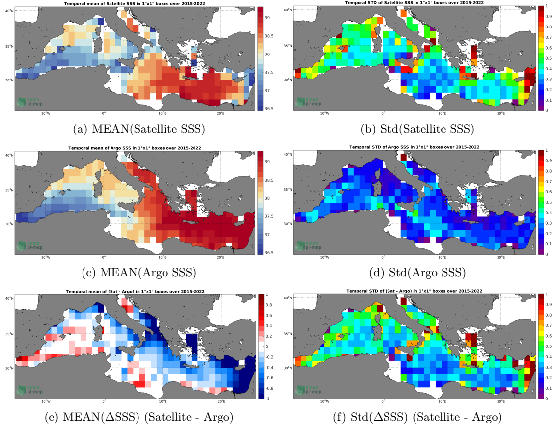
Figure 6: Temporal mean (left) and Std (right) of SSS from SMAP SSS L2-AVERAGED v5.0 (JPL) (top), Argo (middle), and of \Delta\text{SSS} (Satellite - Argo). Only match-up pairs are used to generate these maps.
