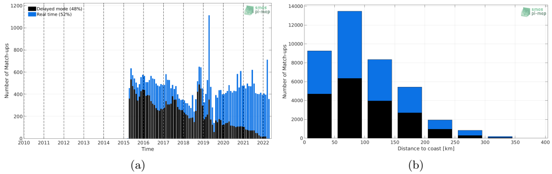
Figure 1: Number of match-ups between Argo and SMAP SSS L2-AVERAGED v5.0 (JPL) SSS as a function of time (a) and as function of the distance to coast (b) over the Mediterranean Sea Pi-MEP region and for the full satellite product period.
