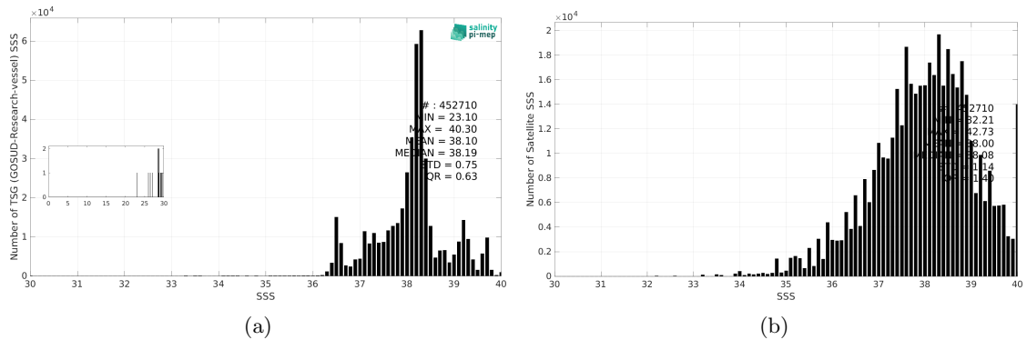
Figure 3: Histograms of SSS from TSG (GOSUD-Research-vessel) (a) and SMAP SSS L2 v6 (RSS) (b) considering all match-up pairs per bins of 0.1 over the Mediterranean Sea Pi-MEP region and for the full satellite product period.
