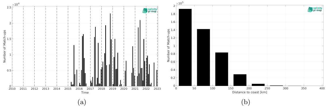
Figure 2: Number of match-ups between TSG (GOSUD-Research-vessel) and SMAP SSS L2 v6 (RSS) SSS as a function of time (a) and as function of the distance to coast (b) over the Mediterranean Sea Pi-MEP region and for the full satellite product period.
