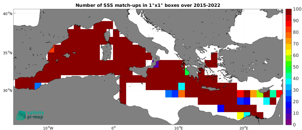
Figure 5: Number of SSS match-ups between TSG (GOSUD-Research-vessel) SSS and the SMAP SSS L2 v6 (RSS) SSS product for the Mediterranean Sea Pi-MEP region over 1^\circ \times 1^\circ boxes and for the full satellite product period.
