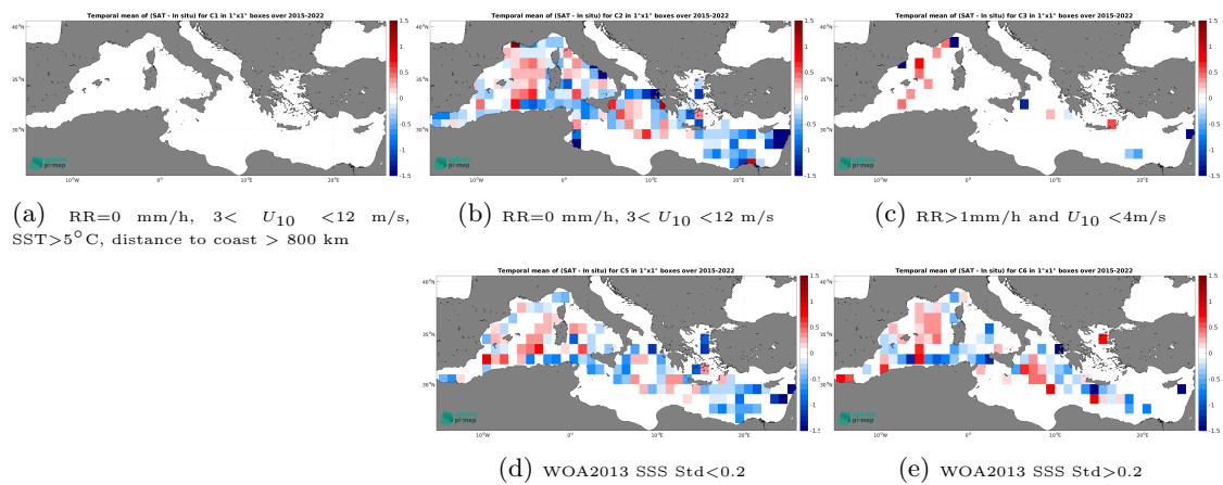
Figure 14: Temporal mean gridded over spatial boxes of size 1^\circ \times 1^\circ of \Delta\text{SSS} (SMAP SSS L2 v6 (RSS) - TSG (GOSUD-Research-vessel)) for 5 different subdatasets corresponding to:RR=0 mm/h, 3 < U_{10} < 12 m/s, SST >5^\circ\text{C} , distance to coast > 800 km (a), RR=0 mm/h, 3 < U_{10} < 12 m/s (b), RR >1 mm/h and U_{10} < 4 m/s (c), WOA2013 SSS Std <0.2 (d), WOA2013 SSS Std >0.2 (e).
