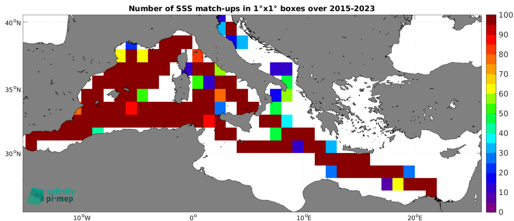
Figure 5: Number of SSS match-ups between TSG (LEGOS-DM) SSS and the SMAP SSS L2 v6 - 40 km (RSS) SSS product for the Mediterranean Sea Pi-MEP region over 1^\circ \times 1^\circ boxes and for the full satellite product period.
