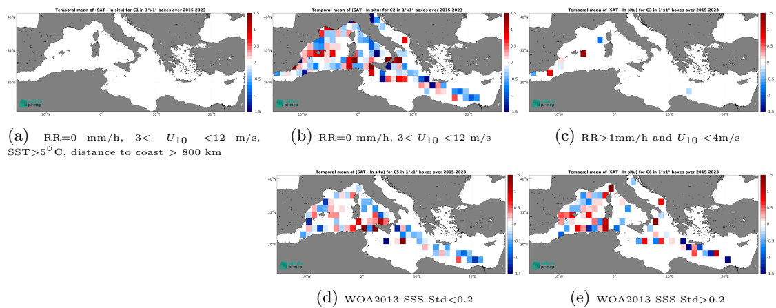
Figure 14: Temporal mean gridded over spatial boxes of size 1^\circ \times 1^\circ of \Delta SSS (SMAP SSS L2 v6 - 40 km (RSS) - TSG (LEGOS-DM)) for 5 different subdatasets corresponding to:RR=0 mm/h, 3 < U_{10} < 12 m/s, SST>5°C, distance to coast > 800 km (a), RR=0 mm/h, 3 < U_{10} < 12 m/s (b), RR>1mm/h and U_{10} < 4 m/s (c), WOA2013 SSS Std<0.2 (d), WOA2013 SSS Std>0.2 (e).
