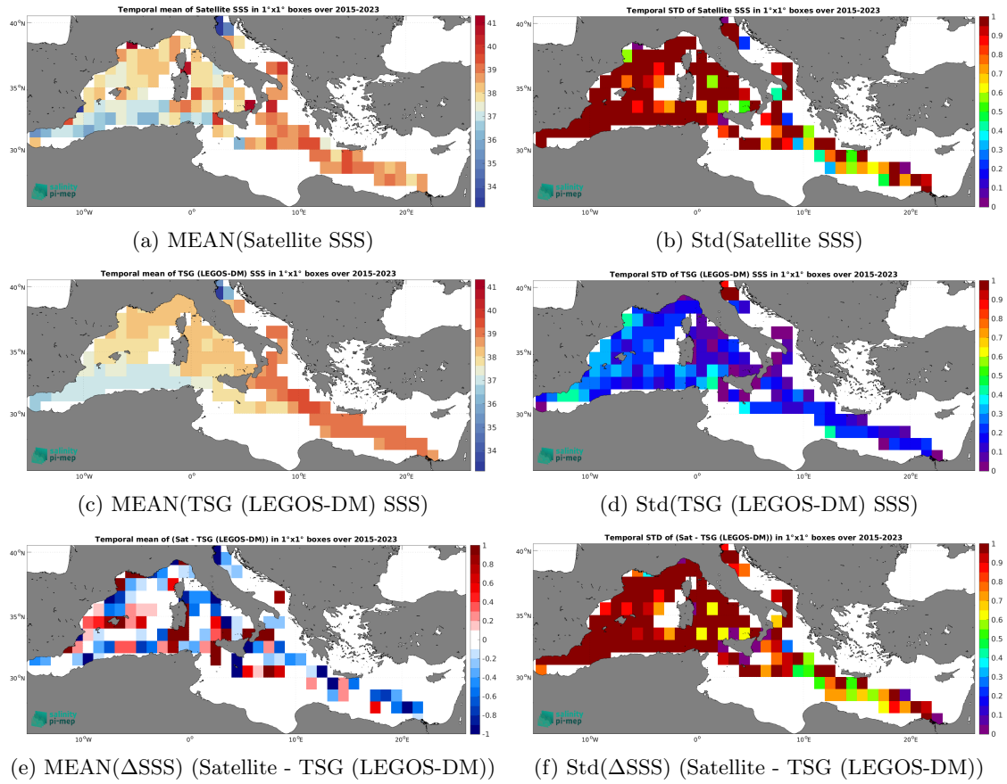
Figure 7: Temporal mean (left) and Std (right) of SSS from SMAP SSS L2 v6 - 40 km (RSS) (top), TSG (LEGOS-DM) (middle), and of \Delta SSS (Satellite - TSG (LEGOS-DM)). Only match-up pairs are used to generate these maps.
