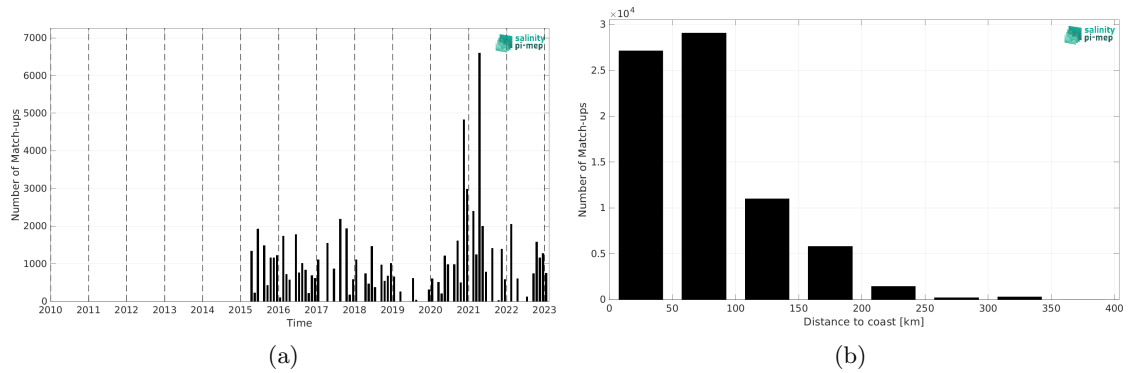
Figure 2: Number of match-ups between TSG (LEGOS-DM) and SMAP SSS L2 v6 - 40 km (RSS) SSS as a function of time (a) and as function of the distance to coast (b) over the Mediterranean Sea Pi-MEP region and for the full satellite product period.
