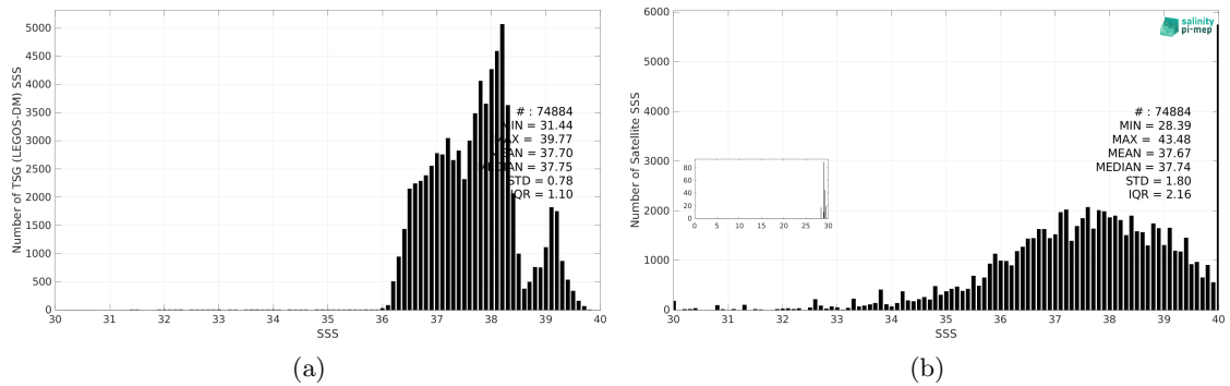
Figure 3: Histograms of SSS from TSG (LEGOS-DM) (a) and SMAP SSS L2 v6 - 40 km (RSS) (b) considering all match-up pairs per bins of 0.1 over the Mediterranean Sea Pi-MEP region and for the full satellite product period.
