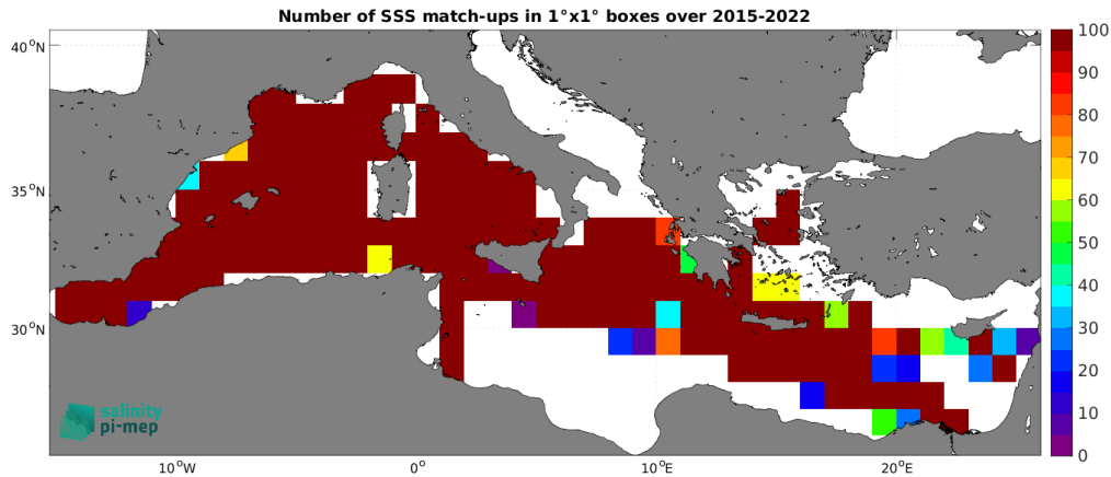
Figure 5: Number of SSS match-ups between TSG (GOSUD-Research-vessel) SSS and the SMAP SSS L2 v6 - 40 km (RSS) SSS product for the Mediterranean Sea Pi-MEP region over 1^\circ \times 1^\circ boxes and for the full satellite product period.
