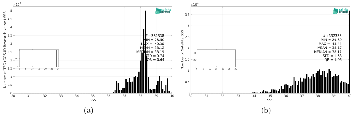
Figure 3: Histograms of SSS from TSG (GOSUD-Research-vessel) (a) and SMAP SSS L2 v6 - 40 km (RSS) (b) considering all match-up pairs per bins of 0.1 over the Mediterranean Sea Pi-MEP region and for the full satellite product period.
