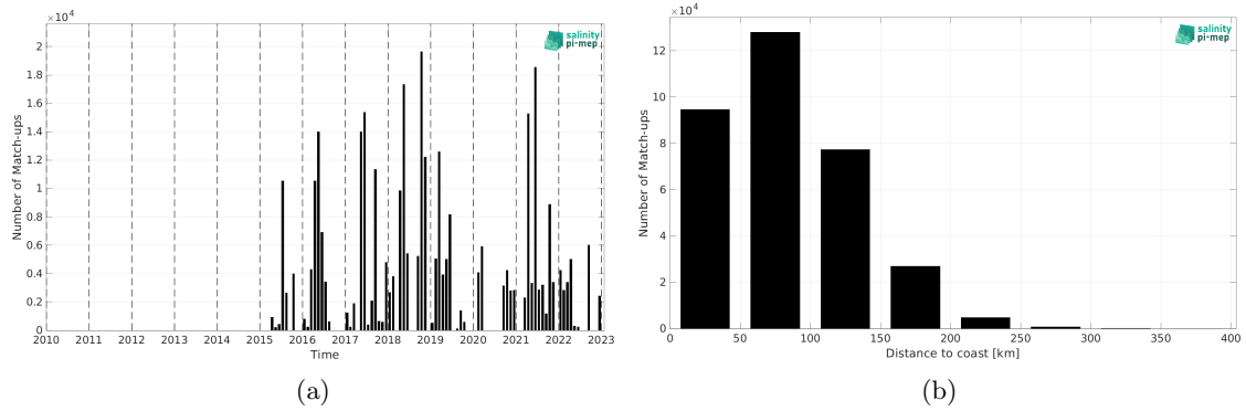
Figure 2: Number of match-ups between TSG (GOSUD-Research-vessel) and SMAP SSS L2 v6 - 40 km (RSS) SSS as a function of time (a) and as function of the distance to coast (b) over the Mediterranean Sea Pi-MEP region and for the full satellite product period.
