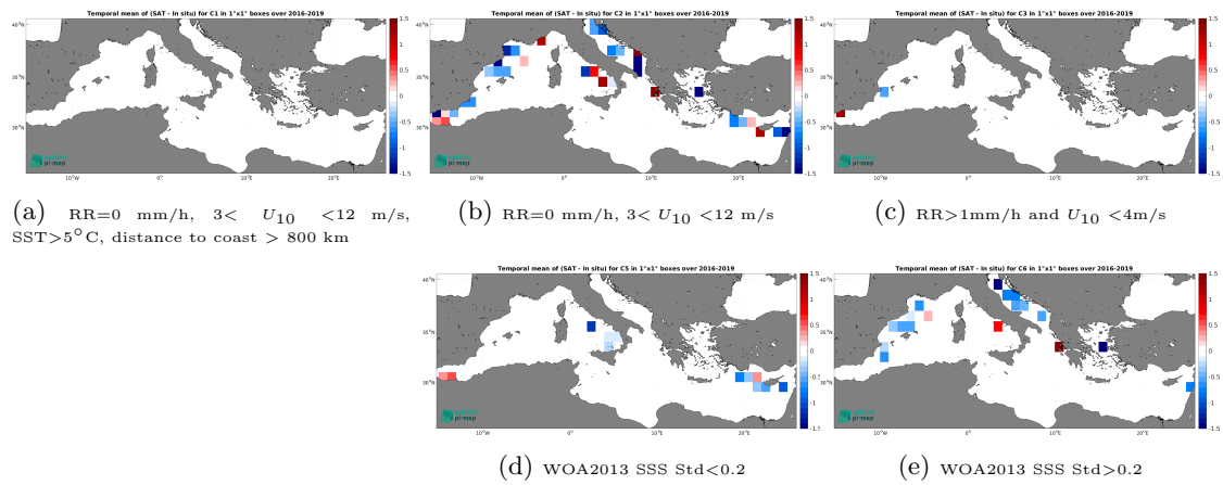
Figure 12: Temporal mean gridded over spatial boxes of size 1^\circ \times 1^\circ of \Delta SSS (SMAP SSS L2 v5 (RSS) - TSG (GOSUD-Sailing-ship)) for 5 different subdatasets corresponding to:RR=0 mm/h, 3 < U_{10} < 12 m/s, SST>5°C, distance to coast > 800 km (a), RR=0 mm/h, 3 < U_{10} < 12 m/s (b), RR>1mm/h and U_{10} < 4 m/s (c), WOA2013 SSS Std<0.2 (d), WOA2013 SSS Std>0.2 (e).
