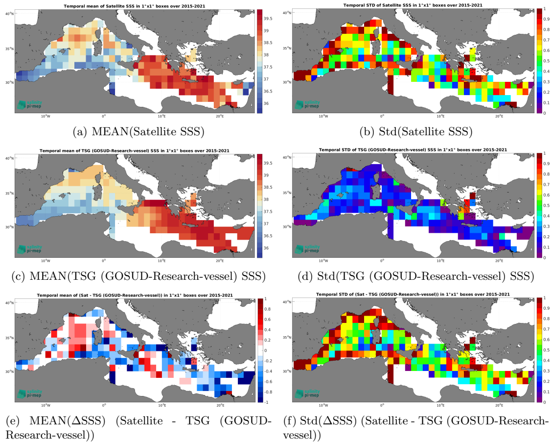
Figure 6: Temporal mean (left) and Std (right) of SSS from SMAP SSS L2 v5 (RSS) (top), TSG (GOSUD-Research-vessel) (middle), and of \Delta SSS (Satellite - TSG (GOSUD-Research-vessel)). Only match-up pairs are used to generate these maps.
