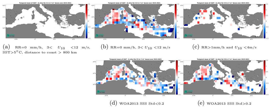
Figure 12: Temporal mean gridded over spatial boxes of size 1^\circ \times 1^\circ of \Delta\text{SSS} (SMAP SSS L2 v5 (RSS) - TSG (GOSUD-Research-vessel)) for 5 different subdatasets corresponding to:RR=0 mm/h, 3 < U_{10} < 12 m/s, SST >5^\circ\text{C} , distance to coast > 800 km (a), RR=0 mm/h, 3 < U_{10} < 12 m/s (b), RR >1 mm/h and U_{10} < 4 m/s (c), WOA2013 SSS Std <0.2 (d), WOA2013 SSS Std >0.2 (e).
