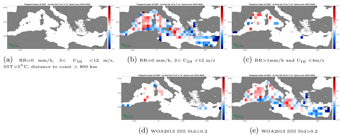
Figure 12: Temporal mean gridded over spatial boxes of size 1^\circ \times 1^\circ of \Delta SSS (SMAP SSS L2 v5 (RSS) - TSG (GOSUD-Research-vessel)) for 5 different subdatasets corresponding to:RR=0 mm/h, 3 < U_{10} < 12 m/s, SST >5^\circ\text{C} , distance to coast > 800 km (a), RR=0 mm/h, 3 < U_{10} < 12 m/s (b), RR >1 mm/h and U_{10} < 4 m/s (c), WOA2013 SSS Std <0.2 (d), WOA2013 SSS Std >0.2 (e).
