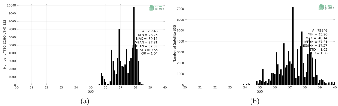
Figure 2: Histograms of SSS from TSG (CSIC-UTM) (a) and SMAP SSS L2 v5 (RSS) (b) considering all match-up pairs per bins of 0.1 over the Mediterranean Sea Pi-MEP region and for the full satellite product period.
