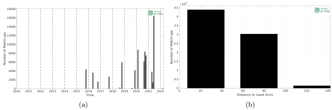
Figure 1: Number of match-ups between TSG (CSIC-UTM) and SMAP SSS L2 v5 (RSS) SSS as a function of time (a) and as function of the distance to coast (b) over the Mediterranean Sea Pi-MEP region and for the full satellite product period.
