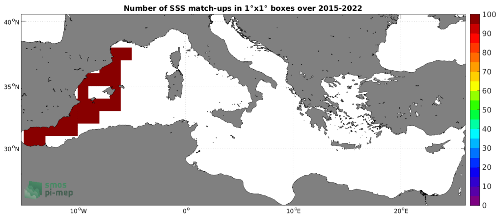
Figure 4: Number of SSS match-ups between TSG (CSIC-UTM) SSS and the SMAP SSS L2 v5 (RSS) SSS product for the Mediterranean Sea Pi-MEP region over 1^\circ \times 1^\circ boxes and for the full satellite product period.
