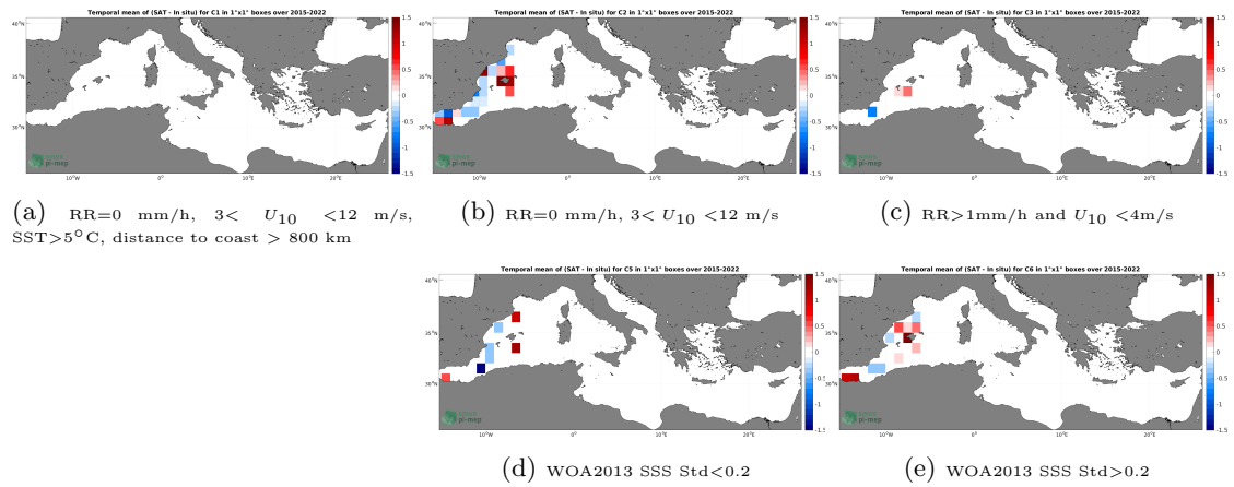
Figure 12: Temporal mean gridded over spatial boxes of size 1^\circ \times 1^\circ of \Delta SSS (SMAP SSS L2 v5 (RSS) - TSG (CSIC-UTM)) for 5 different subdatasets corresponding to:RR=0 mm/h, 3 < U_{10} < 12 m/s, SST >5^\circ\text{C} , distance to coast > 800 km (a), RR=0 mm/h, 3 < U_{10} < 12 m/s (b), RR >1 mm/h and U_{10} < 4 m/s (c), WOA2013 SSS Std <0.2 (d), WOA2013 SSS Std >0.2 (e).
