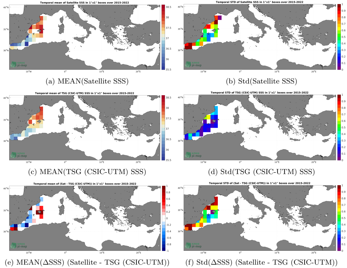
Figure 6: Temporal mean (left) and Std (right) of SSS from SMAP SSS L2 v5 (RSS) (top), TSG (CSIC-UTM) (middle), and of \Delta SSS (Satellite - TSG (CSIC-UTM)). Only match-up pairs are used to generate these maps.
