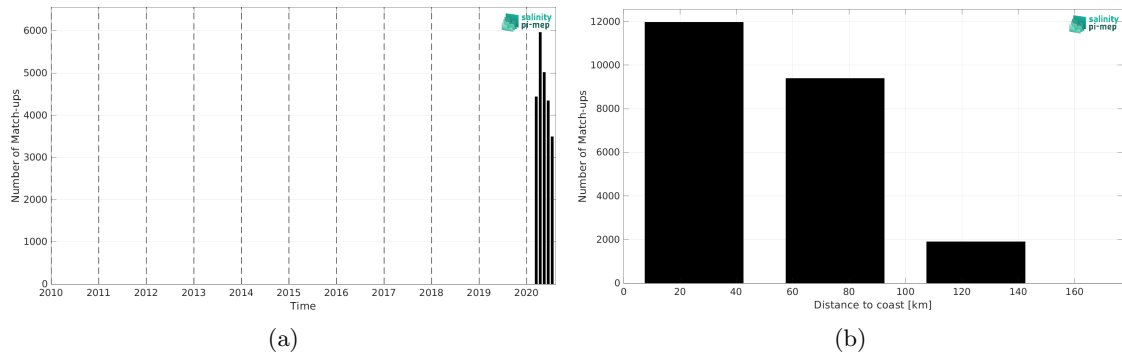
Figure 1: Number of match-ups between Saildrone and SMAP SSS L2 v5 (RSS) SSS as a function of time (a) and as function of the distance to coast (b) over the Mediterranean Sea Pi-MEP region and for the full satellite product period.
