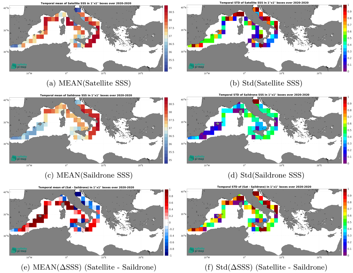
Figure 6: Temporal mean (left) and Std (right) of SSS from SMAP SSS L2 v5 (RSS) (top), Saildrone (middle), and of \Delta SSS (Satellite - Saildrone). Only match-up pairs are used to generate these maps.
