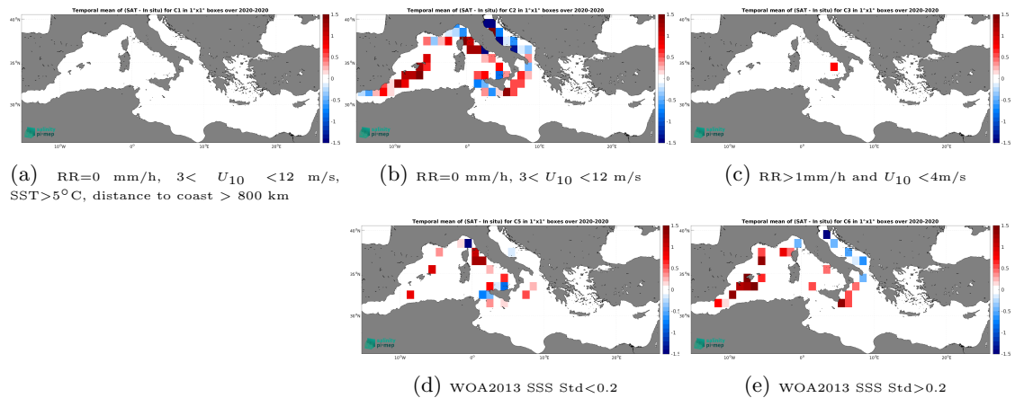
Figure 12: Temporal mean gridded over spatial boxes of size 1^\circ \times 1^\circ of \Delta SSS (SMAP SSS L2 v5 (RSS) - Saldrone) for 5 different subdatasets corresponding to:RR=0 mm/h, 3 < U_{10} < 12 m/s, SST >5^\circ\text{C} , distance to coast > 800 km (a), RR=0 mm/h, 3 < U_{10} < 12 m/s (b), RR >1 mm/h and U_{10} < 4 m/s (c), WOA2013 SSS Std <0.2 (d), WOA2013 SSS Std >0.2 (e).
