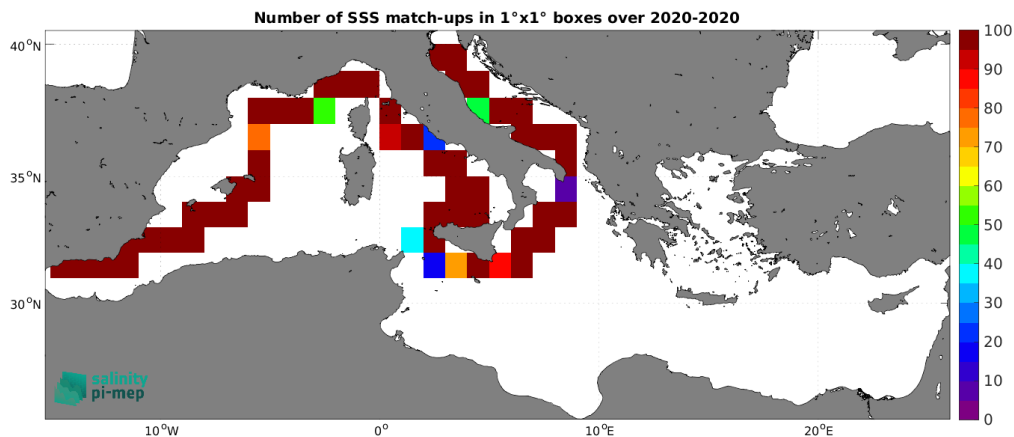
Figure 4: Number of SSS match-ups between Saildrone SSS and the SMAP SSS L2 v5 (RSS) SSS product for the Mediterranean Sea Pi-MEP region over 1^\circ \times 1^\circ boxes and for the full satellite product period.
