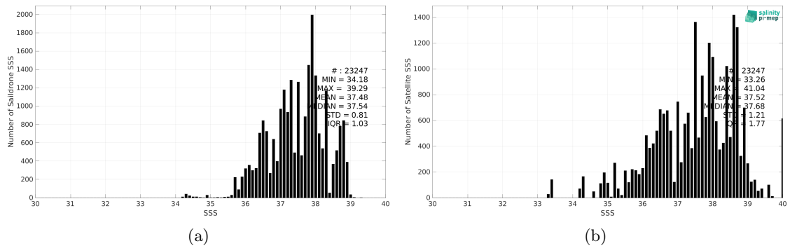
Figure 2: Histograms of SSS from Saildrone (a) and SMAP SSS L2 v5 (RSS) (b) considering all match-up pairs per bins of 0.1 over the Mediterranean Sea Pi-MEP region and for the full satellite product period.
