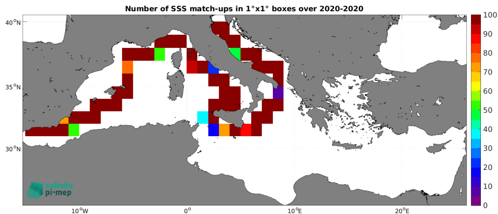
Figure 5: Number of SSS match-ups between Saildrone SSS and the SMAP SSS L2 v5.3 (RSS) SSS product for the Mediterranean Sea Pi-MEP region over 1^\circ \times 1^\circ boxes and for the full satellite product period.
