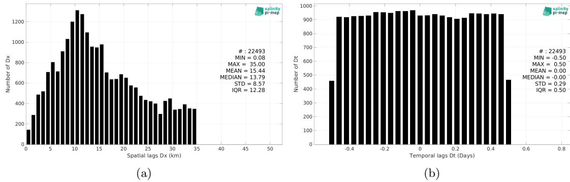
Figure 6: Histograms of the spatial (a) and temporal (b) lags between the location/time of the Saildrone measurement and the date of the corresponding SMAP SSS L2 v5.3 (RSS) SSS pixel.
