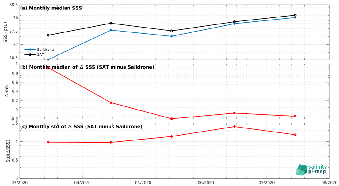
Figure 8: Time series of the monthly median SSS (top), median of \Delta SSS (Satellite - Sairdron) and Std of \Delta SSS (Satellite - Sairdron) over the Mediterranean Sea Pi-MEP region considering all match-ups collected by the Pi-MEP.
