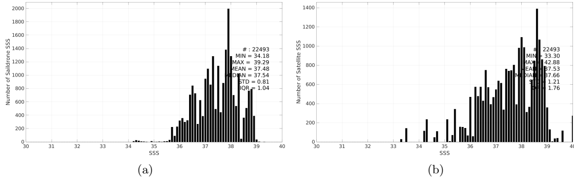
Figure 3: Histograms of SSS from Saildrone (a) and SMAP SSS L2 v5.3 (RSS) (b) considering all match-up pairs per bins of 0.1 over the Mediterranean Sea Pi-MEP region and for the full satellite product period.
