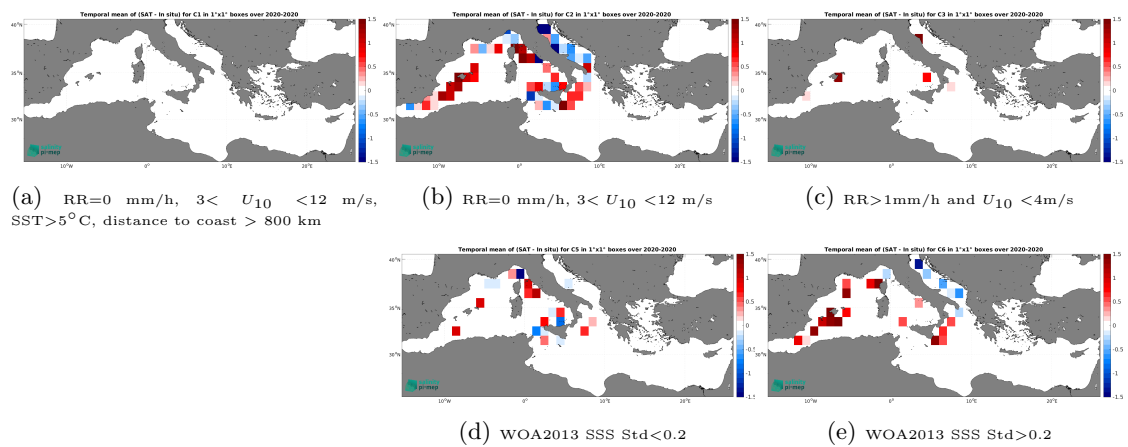
Figure 14: Temporal mean gridded over spatial boxes of size 1^\circ \times 1^\circ of \Delta\text{SSS} (SMAP SSS L2 v5.3 (RSS) - Saildrone) for 5 different subdatasets corresponding to:RR=0 mm/h, 3 < U_{10} < 12 m/s, SST >5^\circ\text{C} , distance to coast > 800 km (a), RR=0 mm/h, 3 < U_{10} < 12 m/s (b), RR >1 mm/h and U_{10} < 4 m/s (c), WOA2013 SSS Std <0.2 (d), WOA2013 SSS Std >0.2 (e).
