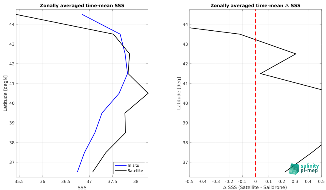
Figure 9: Left panel: Zonal mean SSS from SMAP SSS L2 v5.3 (RSS) satellite product (black) and from Saildrone (blue). Right panel: Zonal mean of \Delta SSS (Satellite - Saildrone) for all the collected Pi-MEP match-up pairs estimated over the full satellite product period.
