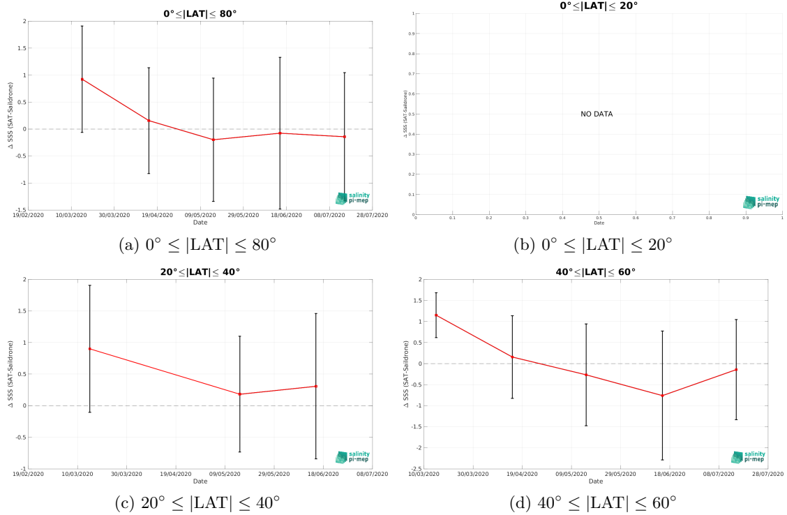
Figure 11: Monthly median (red curves) of \Delta\text{SSS} (Satellite - Saldrone) and \pm 1 Std (black vertical thick bars) as function of time for all the collected Pi-MEP match-up pairs estimated over the Mediterranean Sea Pi-MEP region and for the full satellite product period are shown for different latitude bands: (a) 80°S-80°N, (b) 20°S-20°N, (c) 40°S-20°S and 20°N-40°N and (d) 60°S-40°S and 40°N-60°N.
