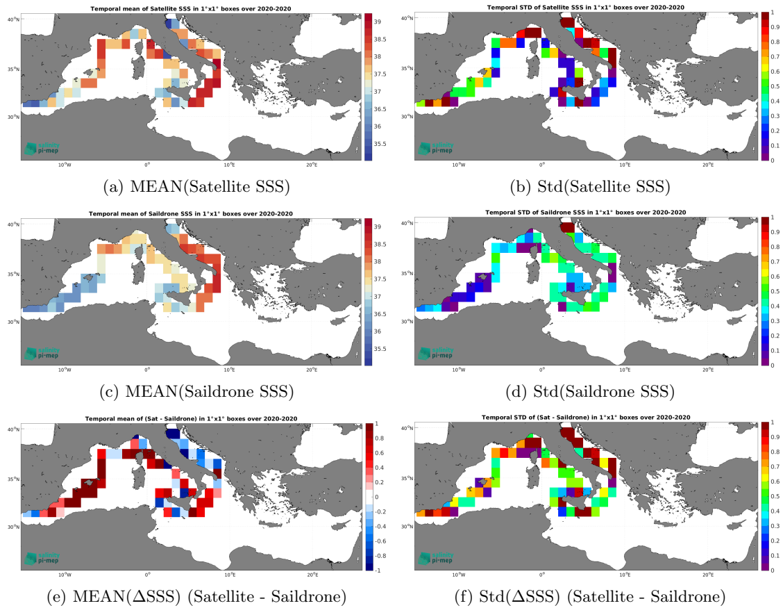
Figure 7: Temporal mean (left) and Std (right) of SSS from SMAP SSS L2 v5.3 (RSS) (top), Saildrone (middle), and of \Delta SSS (Satellite - Saildrone). Only match-up pairs are used to generate these maps.
