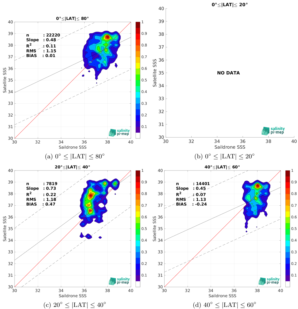
Figure 10: Contour maps of the concentration of SMAP SSS L2 v5.3 (RSS) SSS (y-axis) versus Saildrone SSS (x-axis) at match-up pairs for different latitude bands. For each plot, the red line shows x=y . The black thin and dashed lines indicate a linear fit through the data cloud and the \pm 95\% confidence levels, respectively. The number match-up pairs n , the slope and R^2 coefficient of the linear fit, the root mean square (RMS) and the mean bias between satellite and in situ data are indicated for each latitude band in each plots.
