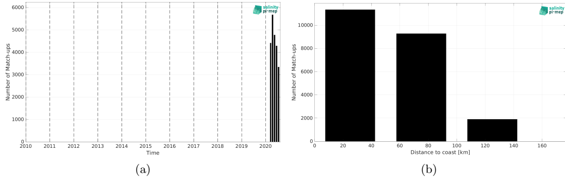
Figure 2: Number of match-ups between Saildrone and SMAP SSS L2 v5.3 (RSS) SSS as a function of time (a) and as function of the distance to coast (b) over the Mediterranean Sea Pi-MEP region and for the full satellite product period.
