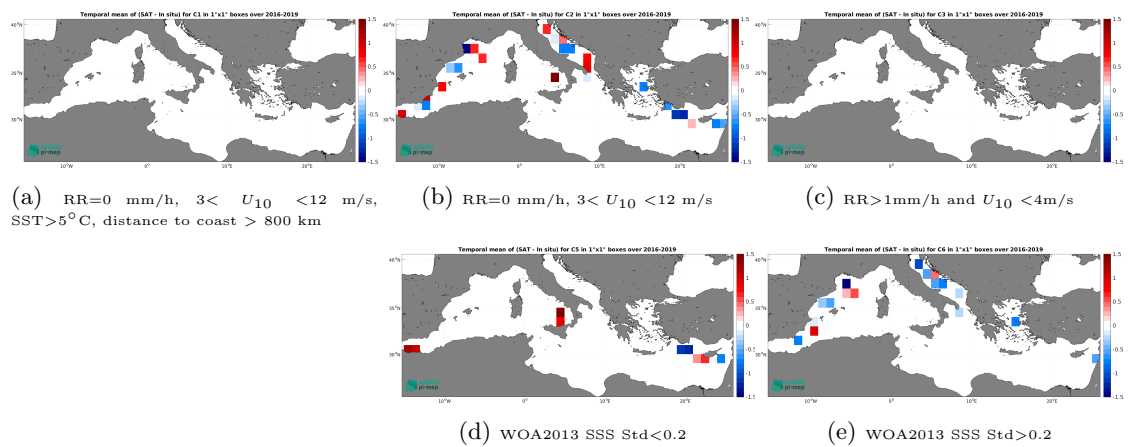
Figure 14: Temporal mean gridded over spatial boxes of size 1^\circ \times 1^\circ of \Delta\text{SSS} (SMAP SSS L2 v5.3 - 40 km (RSS) - TSG (GOSUD-Sailing-ship)) for 5 different subdatasets corresponding to:RR=0 mm/h, 3 < U_{10} < 12 m/s, SST>5°C, distance to coast > 800 km (a), RR=0 mm/h, 3 < U_{10} < 12 m/s (b), RR>1mm/h and U_{10} < 4 m/s (c), WOA2013 SSS Std<0.2 (d), WOA2013 SSS Std>0.2 (e).
