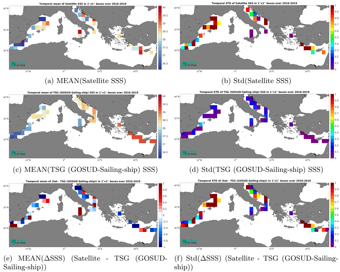
Figure 7: Temporal mean (left) and Std (right) of SSS from SMAP SSS L2 v5.3 - 40 km (RSS) (top), TSG (GOSUD-Sailing-ship) (middle), and of \Delta SSS (Satellite - TSG (GOSUD-Sailing-ship)). Only match-up pairs are used to generate these maps.
