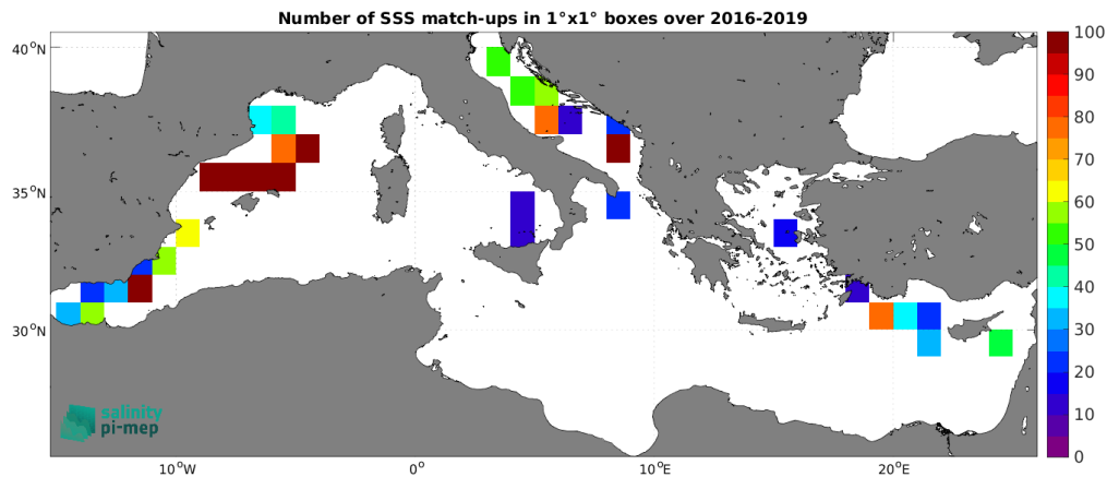
Figure 5: Number of SSS match-ups between TSG (GOSUD-Sailing-ship) SSS and the SMAP SSS L2 v5.3 - 40 km (RSS) SSS product for the Mediterranean Sea Pi-MEP region over 1^\circ \times 1^\circ boxes and for the full satellite product period.
