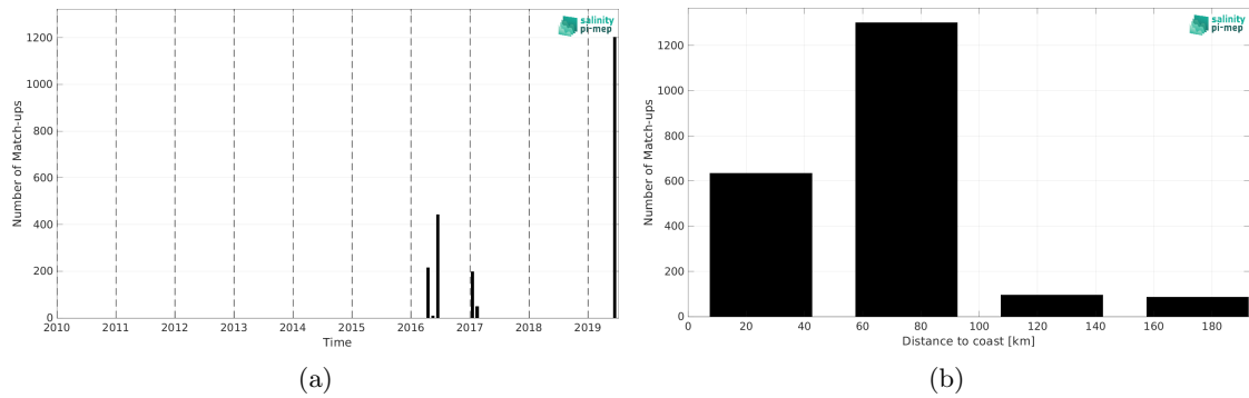
Figure 2: Number of match-ups between TSG (GOSUD-Sailing-ship) and SMAP SSS L2 v5.3 - 40 km (RSS) SSS as a function of time (a) and as function of the distance to coast (b) over the Mediterranean Sea Pi-MEP region and for the full satellite product period.
