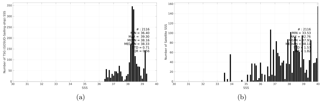
Figure 3: Histograms of SSS from TSG (GOSUD-Sailing-ship) (a) and SMAP SSS L2 v5.3 - 40 km (RSS) (b) considering all match-up pairs per bins of 0.1 over the Mediterranean Sea Pi-MEP region and for the full satellite product period.
