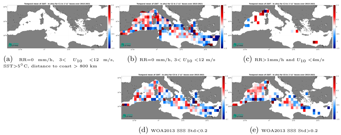
Figure 14: Temporal mean gridded over spatial boxes of size 1^\circ \times 1^\circ of \Delta SSS (SMAP SSS L2 v5.3 - 40 km (RSS) - TSG (GOSUD-Research-vessel)) for 5 different subdatasets corresponding to:RR=0 mm/h, 3 < U_{10} < 12 m/s, SST>5°C, distance to coast > 800 km (a), RR=0 mm/h, 3 < U_{10} < 12 m/s (b), RR>1mm/h and U_{10} < 4 m/s (c), WOA2013 SSS Std<0.2 (d), WOA2013 SSS Std>0.2 (e).
