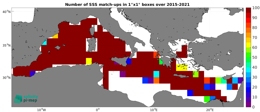
Figure 5: Number of SSS match-ups between TSG (GOSUD-Research-vessel) SSS and the SMAP SSS L2 v5.3 - 40 km (RSS) SSS product for the Mediterranean Sea Pi-MEP region over 1^\circ \times 1^\circ boxes and for the full satellite product period.
