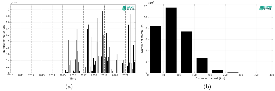
Figure 2: Number of match-ups between TSG (GOSUD-Research-vessel) and SMAP SSS L2 v5.3 - 40 km (RSS) SSS as a function of time (a) and as function of the distance to coast (b) over the Mediterranean Sea Pi-MEP region and for the full satellite product period.
