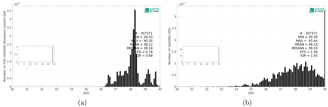
Figure 3: Histograms of SSS from TSG (GOSUD-Research-vessel) (a) and SMAP SSS L2 v5.3 - 40 km (RSS) (b) considering all match-up pairs per bins of 0.1 over the Mediterranean Sea Pi-MEP region and for the full satellite product period.
