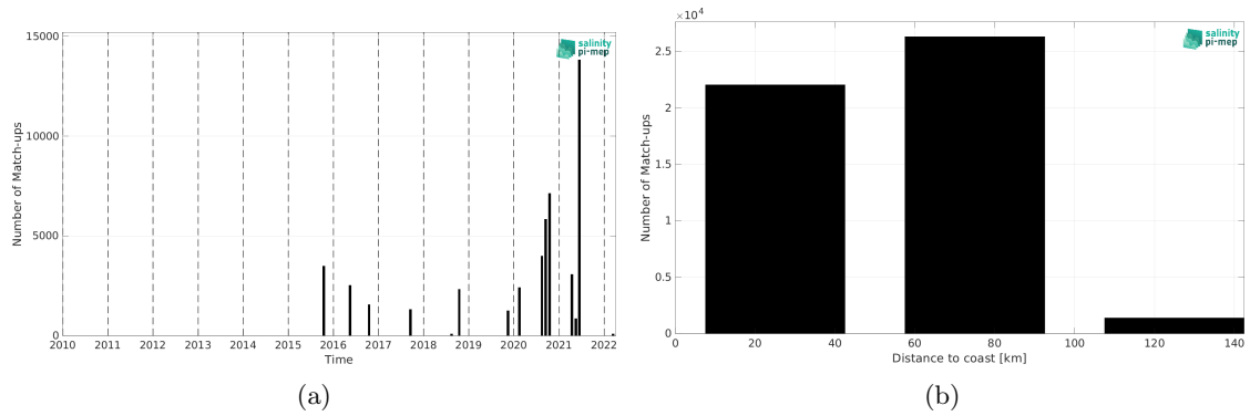
Figure 2: Number of match-ups between TSG (CSIC-UTM) and SMAP SSS L2 v5.3 - 40 km (RSS) SSS as a function of time (a) and as function of the distance to coast (b) over the Mediterranean Sea Pi-MEP region and for the full satellite product period.
