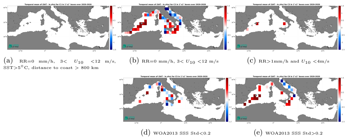
Figure 14: Temporal mean gridded over spatial boxes of size 1^\circ \times 1^\circ of \Delta\text{SSS} (SMAP SSS L2 v5.3 - 40 km (RSS) - Saildrone) for 5 different subdatasets corresponding to:RR=0 mm/h, 3 < U_{10} < 12 m/s, SST >5^\circ\text{C} , distance to coast > 800 km (a), RR=0 mm/h, 3 < U_{10} < 12 m/s (b), RR >1 mm/h and U_{10} < 4 m/s (c), WOA2013 SSS Std <0.2 (d), WOA2013 SSS Std >0.2 (e).
