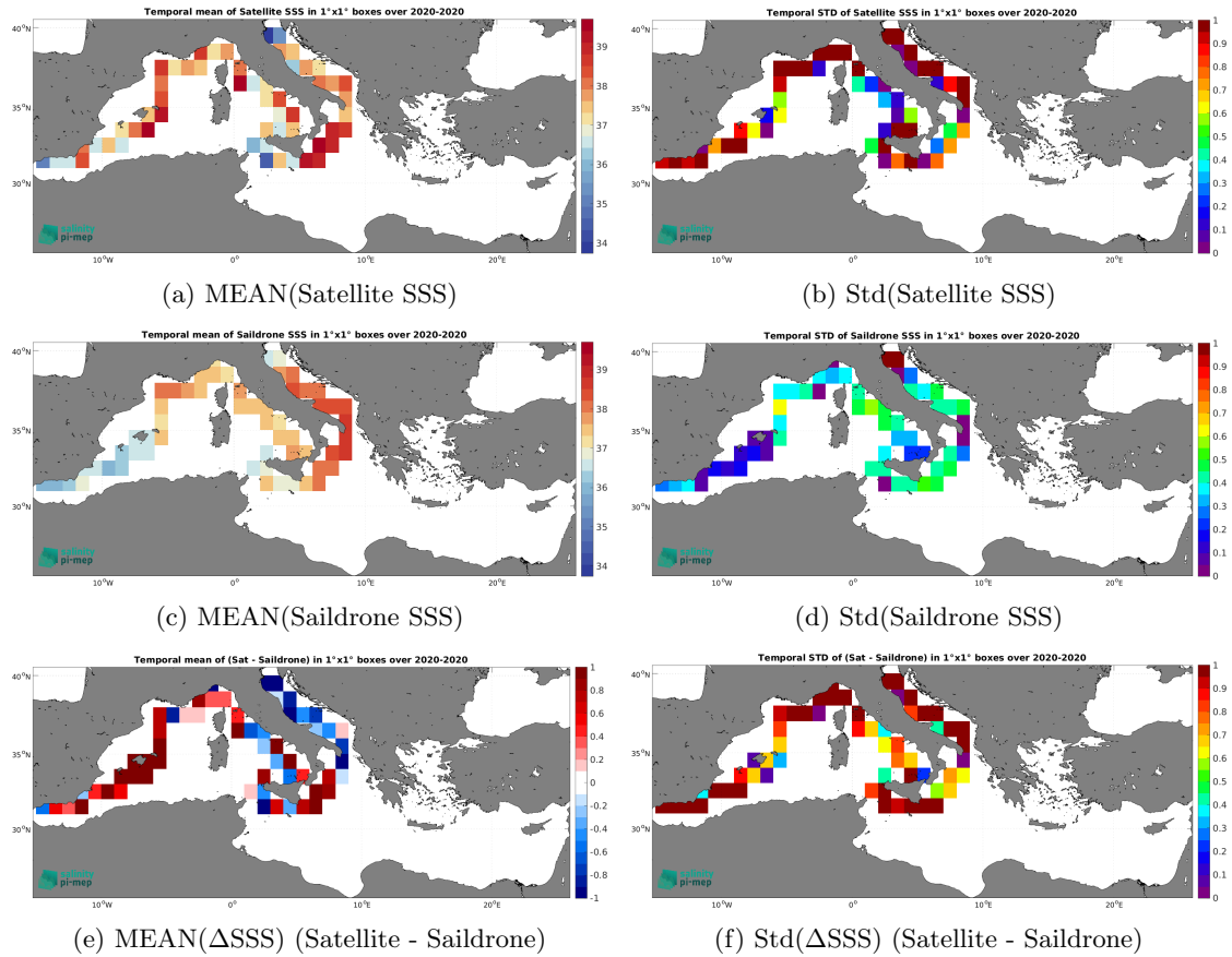
Figure 7: Temporal mean (left) and Std (right) of SSS from SMAP SSS L2 v5.3 - 40 km (RSS) (top), Saildrone (middle), and of \Delta SSS (Satellite - Saildrone). Only match-up pairs are used to generate these maps.
