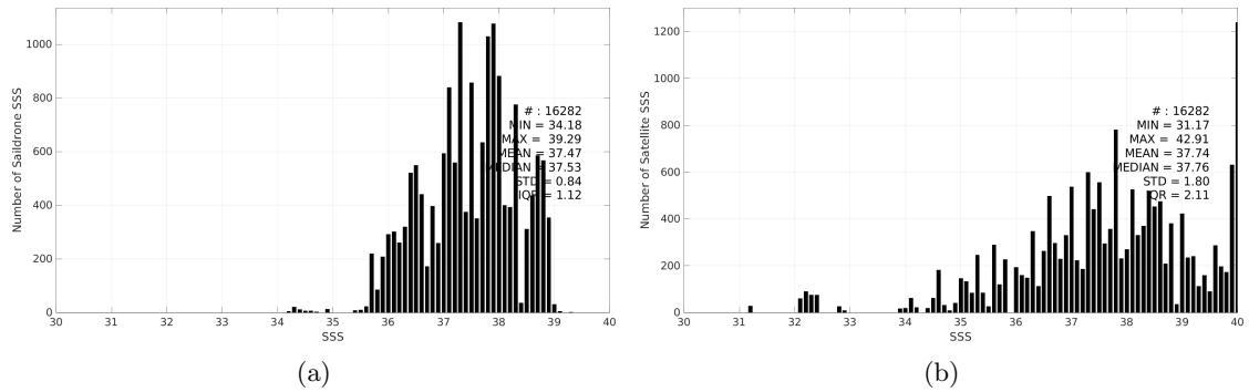
Figure 3: Histograms of SSS from Sailldrone (a) and SMAP SSS L2 v5.3 - 40 km (RSS) (b) considering all match-up pairs per bins of 0.1 over the Mediterranean Sea Pi-MEP region and for the full satellite product period.
