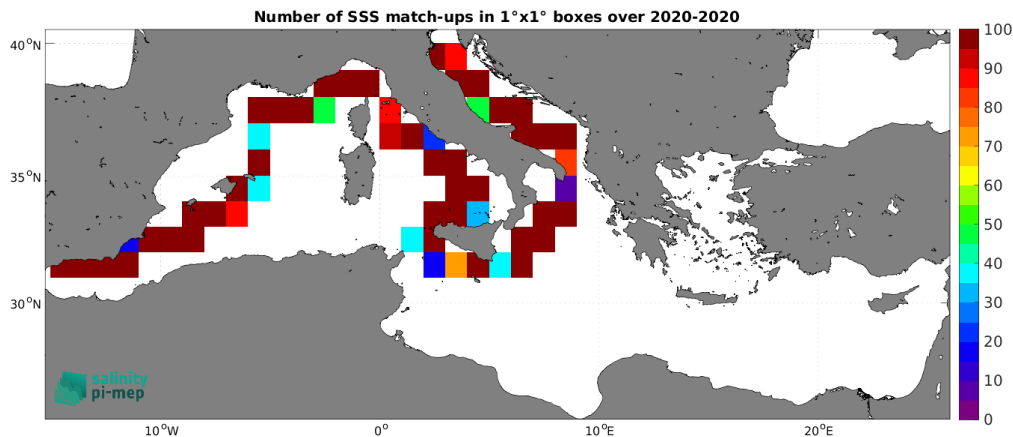
Figure 5: Number of SSS match-ups between Saildrone SSS and the SMAP SSS L2 v5.3 - 40 km (RSS) SSS product for the Mediterranean Sea Pi-MEP region over 1^\circ \times 1^\circ boxes and for the full satellite product period.
