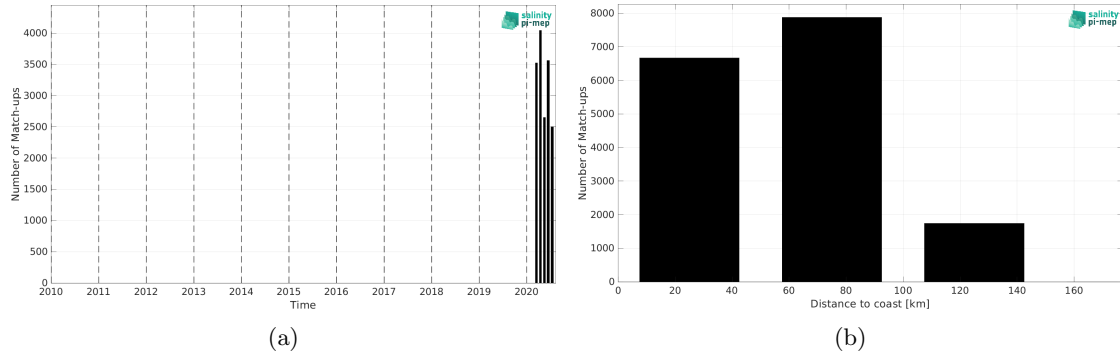
Figure 2: Number of match-ups between Sailldrone and SMAP SSS L2 v5.3 - 40 km (RSS) SSS as a function of time (a) and as function of the distance to coast (b) over the Mediterranean Sea Pi-MEP region and for the full satellite product period.
