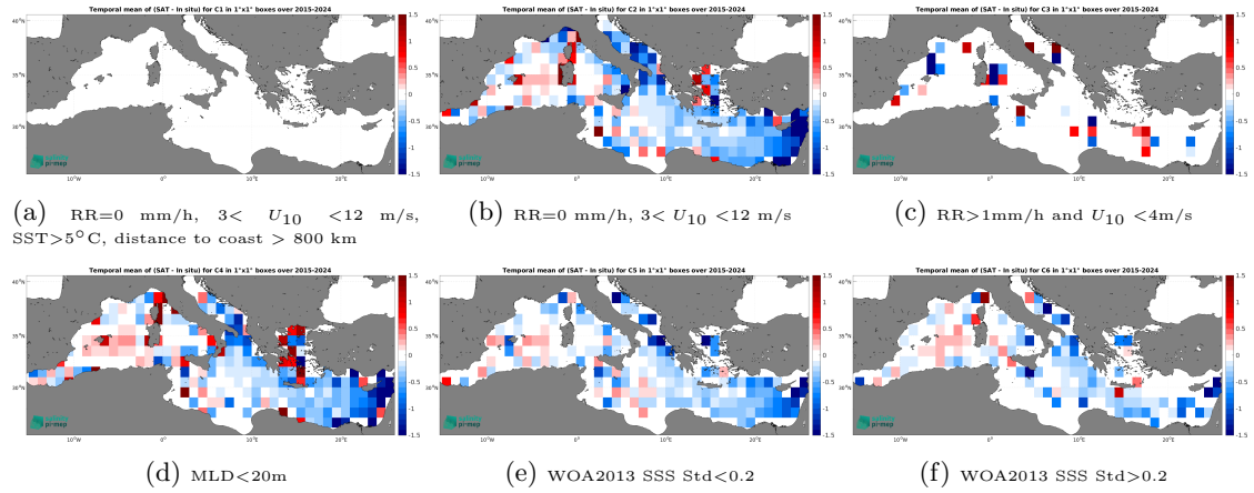
Figure 14: Temporal mean gridded over spatial boxes of size 1^\circ \times 1^\circ of \Delta SSS (SMAP SSS L2 v5.3 - 40 km (RSS) - Argo) for 6 different subdatasets corresponding to:RR=0 mm/h, 3 < U_{10} < 12 m/s, SST>5°C, distance to coast > 800 km (a), RR=0 mm/h, 3 < U_{10} < 12 m/s (b), RR>1mm/h and U_{10} < 4 m/s (c),MLD<20m (d),WOA2013 SSS Std<0.2 (e),WOA2013 SSS Std>0.2 (f).
