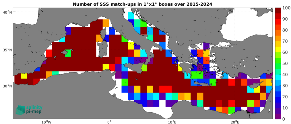
Figure 5: Number of SSS match-ups between Argo SSS and the SMAP SSS L2 v5.3 - 40 km (RSS) SSS product for the Mediterranean Sea Pi-MEP region over 1^\circ \times 1^\circ boxes and for the full satellite product period.
