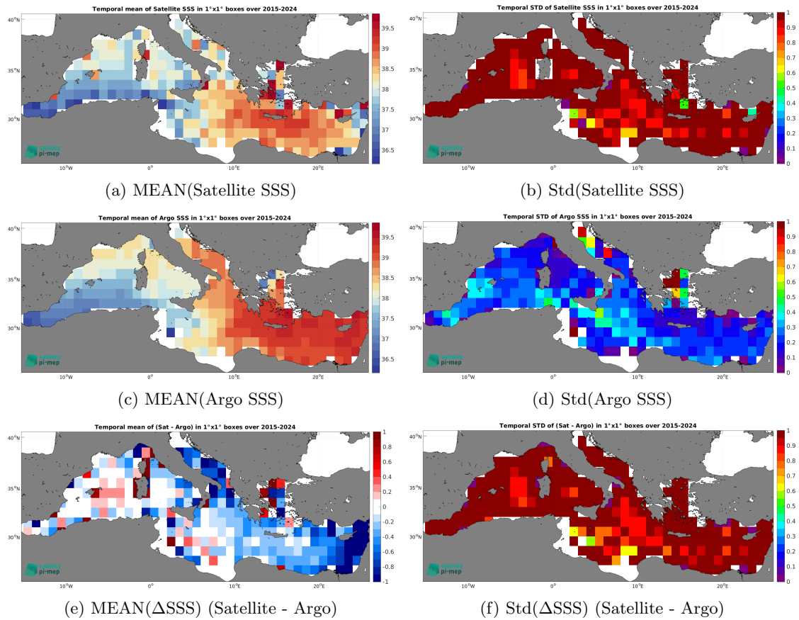
Figure 7: Temporal mean (left) and Std (right) of SSS from SMAP SSS L2 v5.3 - 40 km (RSS) (top), Argo (middle), and of \Delta SSS (Satellite - Argo). Only match-up pairs are used to generate these maps.
