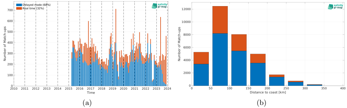
Figure 2: Number of match-ups between Argo and SMAP SSS L2 v5.3 - 40 km (RSS) SSS as a function of time (a) and as function of the distance to coast (b) over the Mediterranean Sea Pi-MEP region and for the full satellite product period.
