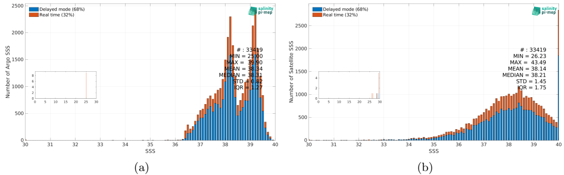
Figure 3: Histograms of SSS from Argo (a) and SMAP SSS L2 v5.3 - 40 km (RSS) (b) considering all match-up pairs per bins of 0.1 over the Mediterranean Sea Pi-MEP region and for the full satellite product period.
