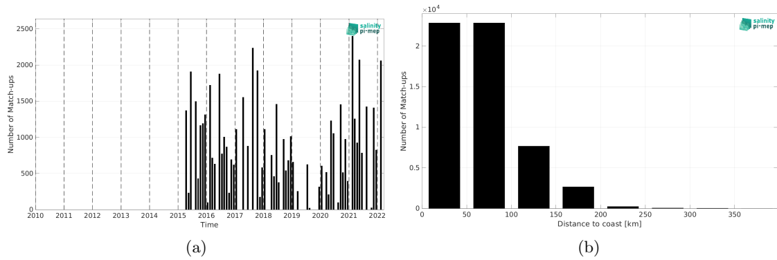
Figure 1: Number of match-ups between TSG (LEGOS-DM) and SMAP SSS L2 v5 - 40 km (RSS) SSS as a function of time (a) and as function of the distance to coast (b) over the Mediterranean Sea Pi-MEP region and for the full satellite product period.
