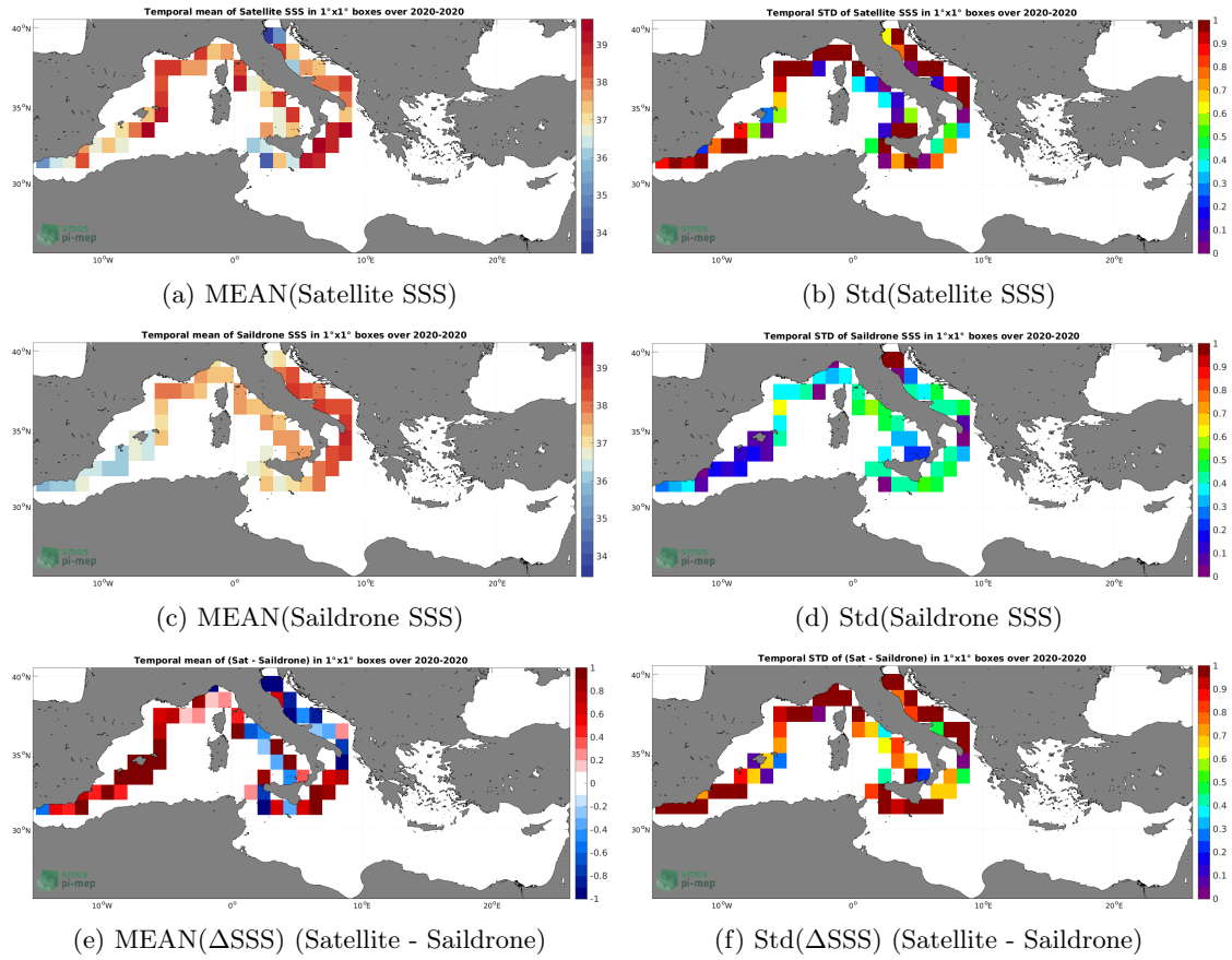
Figure 6: Temporal mean (left) and Std (right) of SSS from SMAP SSS L2 v5 - 40 km (RSS) (top), Saildrone (middle), and of \Delta SSS (Satellite - Saildrone). Only match-up pairs are used to generate these maps.
