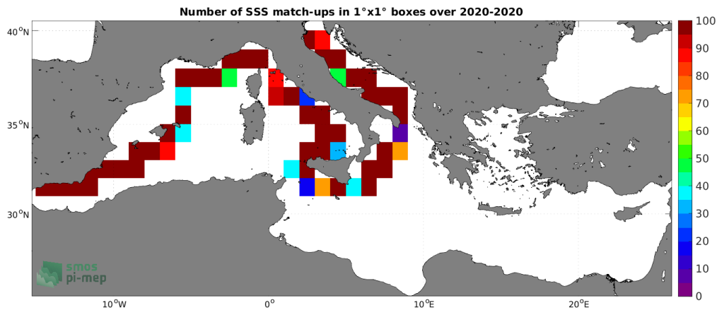
Figure 4: Number of SSS match-ups between Saildrone SSS and the SMAP SSS L2 v5 - 40 km (RSS) SSS product for the Mediterranean Sea Pi-MEP region over 1^\circ \times 1^\circ boxes and for the full satellite product period.
