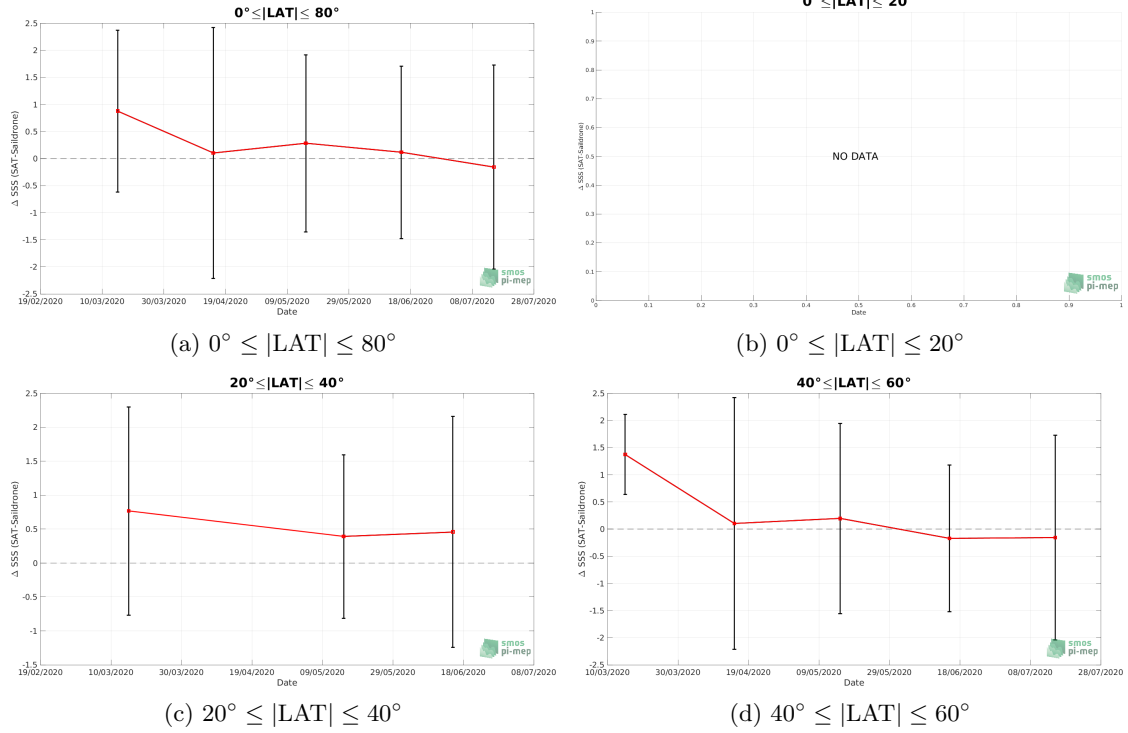
Figure 10: Monthly median (red curves) of \Delta\text{SSS} (Satellite - Saldrone) and \pm 1 Std (black vertical thick bars) as function of time for all the collected Pi-MEP match-up pairs estimated over the Mediterranean Sea Pi-MEP region and for the full satellite product period are shown for different latitude bands: (a) 80°S-80°N, (b) 20°S-20°N, (c) 40°S-20°S and 20°N-40°N and (d) 60°S-40°S and 40°N-60°N.
