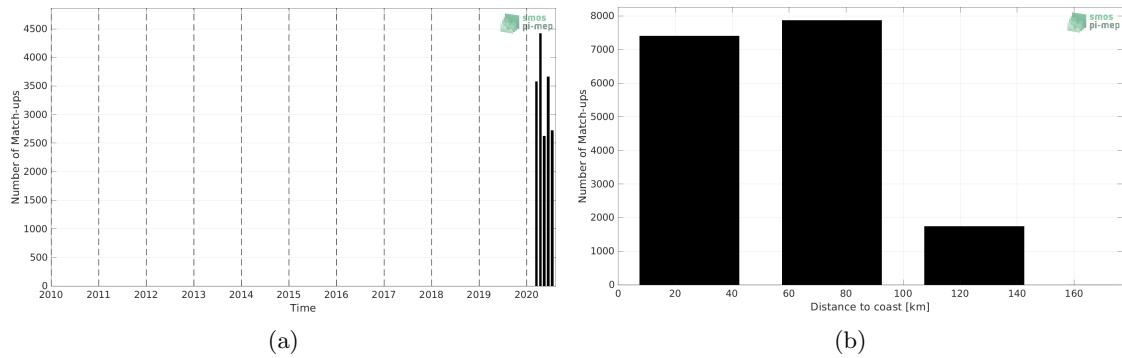
Figure 1: Number of match-ups between Sairdrone and SMAP SSS L2 v5 - 40 km (RSS) SSS as a function of time (a) and as function of the distance to coast (b) over the Mediterranean Sea Pi-MEP region and for the full satellite product period.
