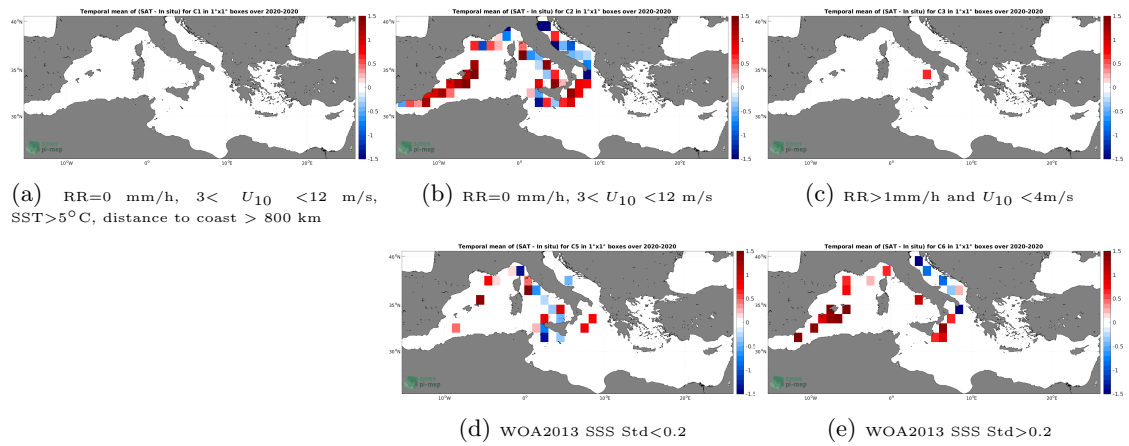
Figure 12: Temporal mean gridded over spatial boxes of size 1^\circ \times 1^\circ of \Delta SSS (SMAP SSS L2 v5 - 40 km (RSS) - Saildrone) for 5 different subdatasets corresponding to:RR=0 mm/h, 3 < U_{10} < 12 m/s, SST >5^\circ\text{C} , distance to coast > 800 km (a), RR=0 mm/h, 3 < U_{10} < 12 m/s (b), RR >1 mm/h and U_{10} < 4 m/s (c), WOA2013 SSS Std <0.2 (d), WOA2013 SSS Std >0.2 (e).
