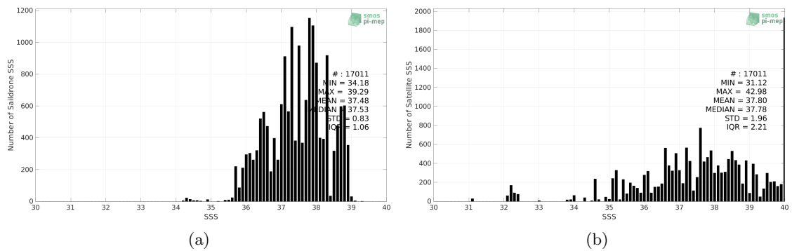
Figure 2: Histograms of SSS from Sairdrone (a) and SMAP SSS L2 v5 - 40 km (RSS) (b) considering all match-up pairs per bins of 0.1 over the Mediterranean Sea Pi-MEP region and for the full satellite product period.
