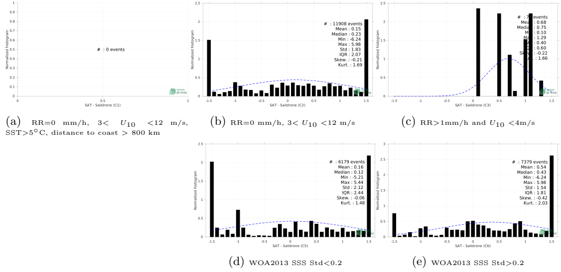
Figure 13: Normalized histogram of \Delta SSS (SMAP SSS L2 v5 - 40 km (RSS) - Saildrone) for 5 different subdatasets corresponding to: RR=0 mm/h, 3 < U_{10} < 12 m/s, SST > 5°C, distance to coast > 800 km (a), RR=0 mm/h, 3 < U_{10} < 12 m/s (b), RR > 1mm/h and U_{10} < 4 m/s (c), WOA2013 SSS Std < 0.2 (d), WOA2013 SSS Std > 0.2 (e).
