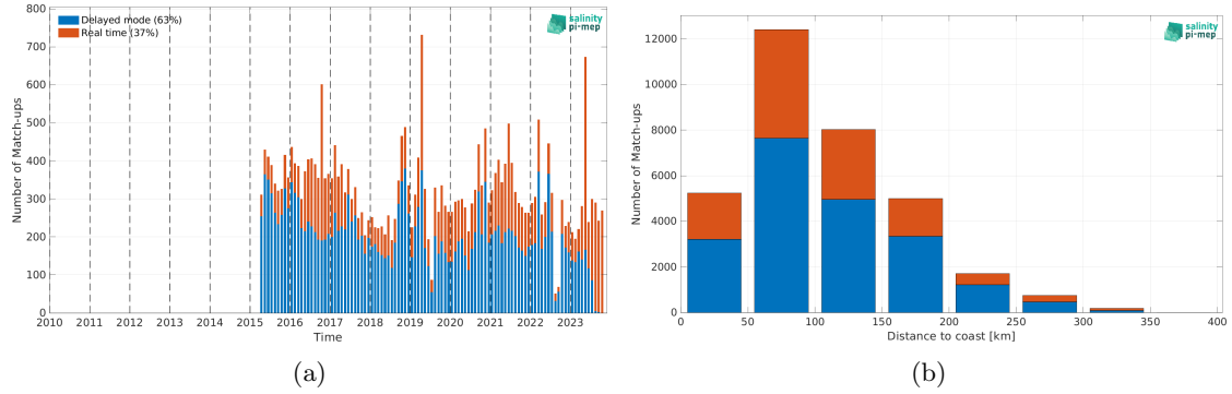
Figure 1: Number of match-ups between Argo and SMAP SSS L2 v5 - 40 km (RSS) SSS as a function of time (a) and as function of the distance to coast (b) over the Mediterranean Sea Pi-MEP region and for the full satellite product period.
