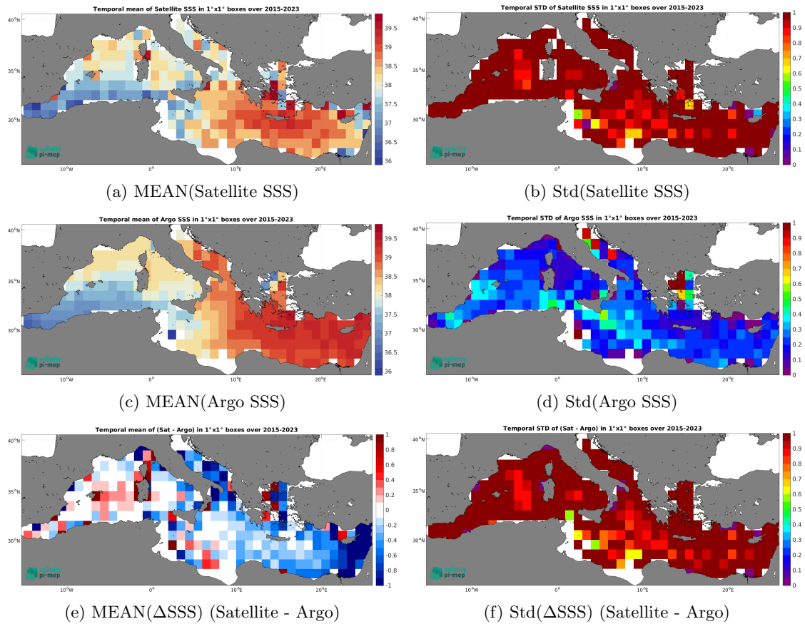
Figure 6: Temporal mean (left) and Std (right) of SSS from SMAP SSS L2 v5 - 40 km (RSS) (top), Argo (middle), and of \Delta SSS (Satellite - Argo). Only match-up pairs are used to generate these maps.
