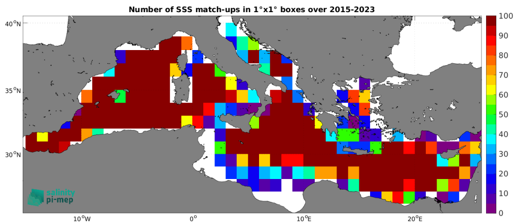
Figure 4: Number of SSS match-ups between Argo SSS and the SMAP SSS L2 v5 - 40 km (RSS) SSS product for the Mediterranean Sea Pi-MEP region over 1^\circ \times 1^\circ boxes and for the full satellite product period.
