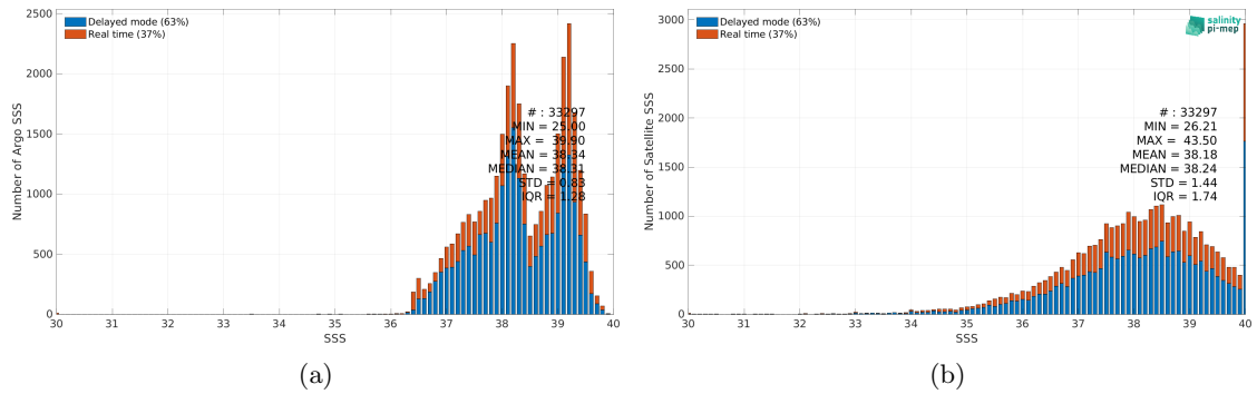
Figure 2: Histograms of SSS from Argo (a) and SMAP SSS L2 v5 - 40 km (RSS) (b) considering all match-up pairs per bins of 0.1 over the Mediterranean Sea Pi-MEP region and for the full satellite product period.
