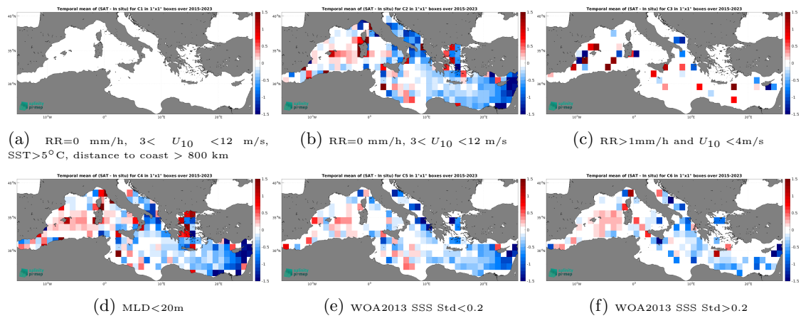
Figure 12: Temporal mean gridded over spatial boxes of size 1^\circ \times 1^\circ of \Delta SSS (SMAP SSS L2 v5 - 40 km (RSS) - Argo) for 6 different subdatasets corresponding to:RR=0 mm/h, 3 < U_{10} < 12 m/s, SST >5^\circ C, distance to coast > 800 km (a), RR=0 mm/h, 3 < U_{10} < 12 m/s (b), RR >1 mm/h and U_{10} < 4 m/s (c),MLD <20 m (d),WOA2013 SSS Std <0.2 (e),WOA2013 SSS Std >0.2 (f).
