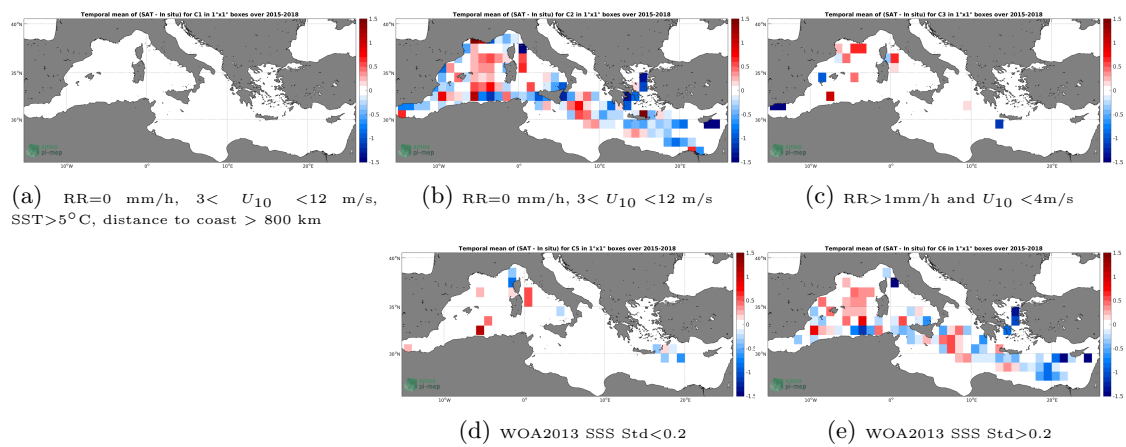
Figure 12: Temporal mean gridded over spatial boxes of size 1^\circ \times 1^\circ of \Delta SSS (SMAP-L2-RSS-V4 - TSG-GOSUD-Research-vessel) for 5 different subdatasets corresponding to:RR=0 mm/h, 3 < U_{10} < 12 m/s, SST >5^\circ\text{C} , distance to coast > 800 km (a), RR=0 mm/h, 3 < U_{10} < 12 m/s (b), RR >1 mm/h and U_{10} < 4 m/s (c), WOA2013 SSS Std <0.2 (d), WOA2013 SSS Std >0.2 (e).
