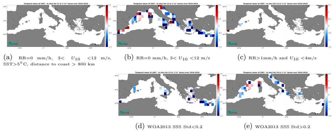
Figure 12: Temporal mean gridded over spatial boxes of size 1^\circ \times 1^\circ of \Delta\text{SSS} (SMAP SSS L2 v5.0 (JPL) - TSG (GOSUD-Sailing-ship)) for 5 different subdatasets corresponding to:RR=0 mm/h, 3 < U_{10} < 12 m/s, SST>5°C, distance to coast > 800 km (a), RR=0 mm/h, 3 < U_{10} < 12 m/s (b), RR>1mm/h and U_{10} < 4 m/s (c), WOA2013 SSS Std<0.2 (d), WOA2013 SSS Std>0.2 (e).
